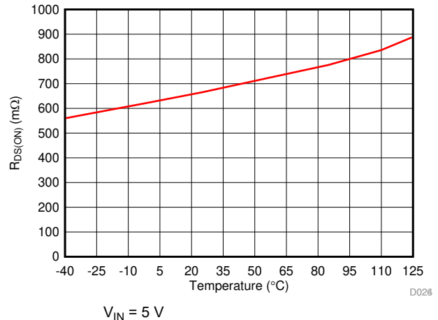
图 8-12. R_{DS(ON)} of High Side MOSFET vs Temperature
