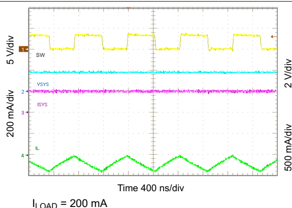
图 10-31. Light Load Operation Showing SW
