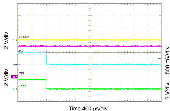
图 10-61. \overline{PG} Functions as Shifted \overline{MR} Output
