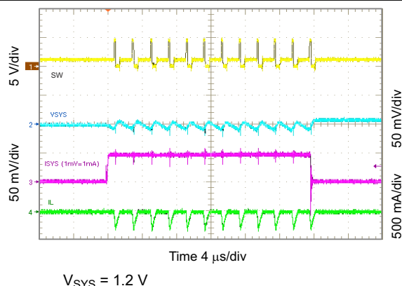
图 10-33. 1.2 V SYS Load Transient, 0 to 50 mA
