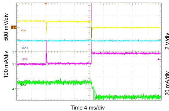
图 10-6. Entering Battery Supplement Mode
