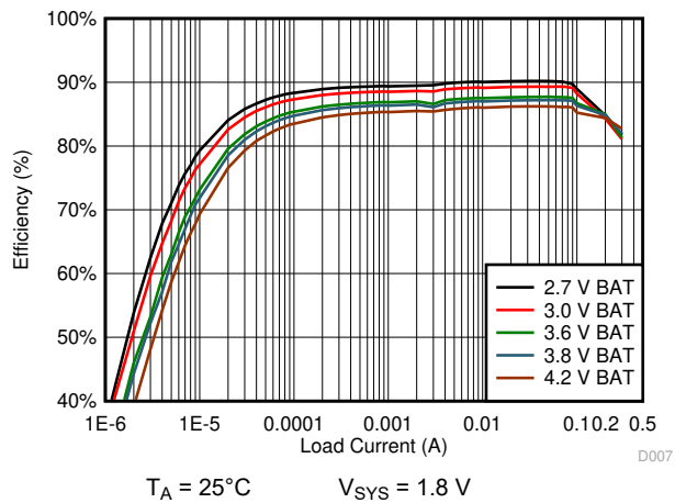
图 10-12. 1.8 V_{\text{SYS}} System Efficiency
