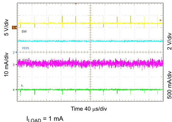
图 10-28. Light Load Operation Showing SW
