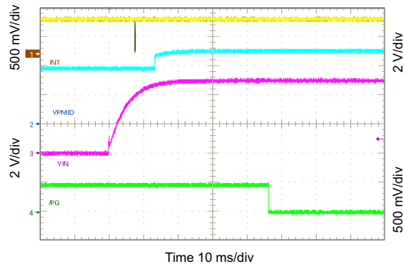
图 10-59. Show \overline{PG} and \overline{INT} Timing ( V_{IN} Insertion)
