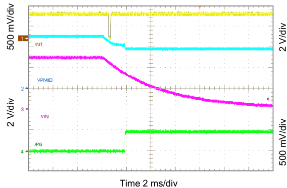
图 10-60. Show \overline{PG} and \overline{INT} Timing ( V_{IN} Removal)
