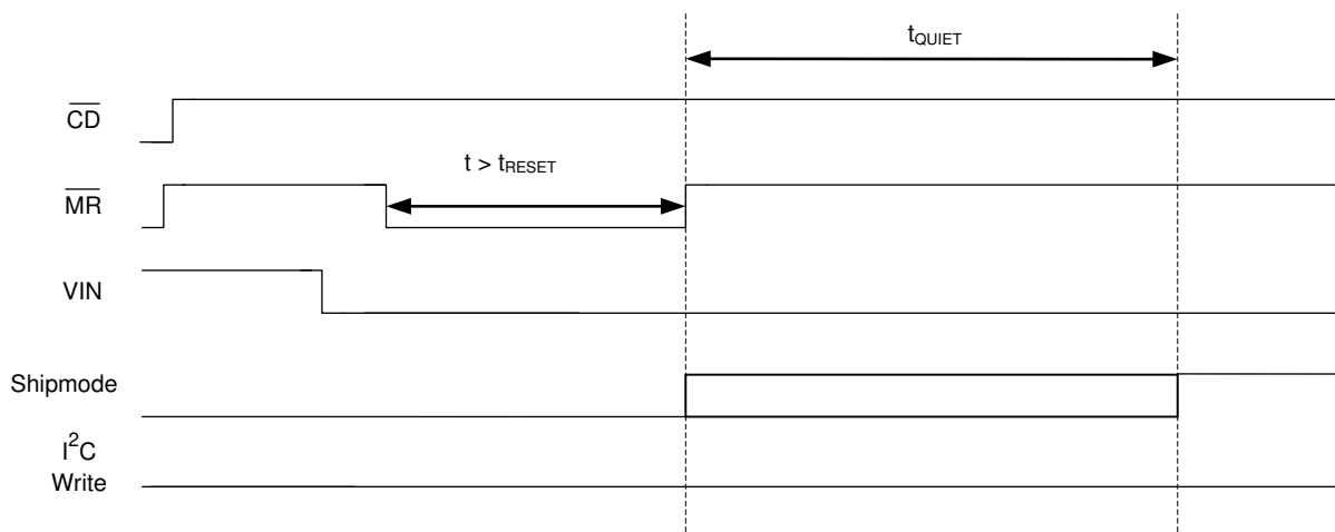
图 9-2. \overline{CD} , \overline{MR} and V_{IN} Sequencing for Ship Mode Entry Through Long \overline{MR} button press
