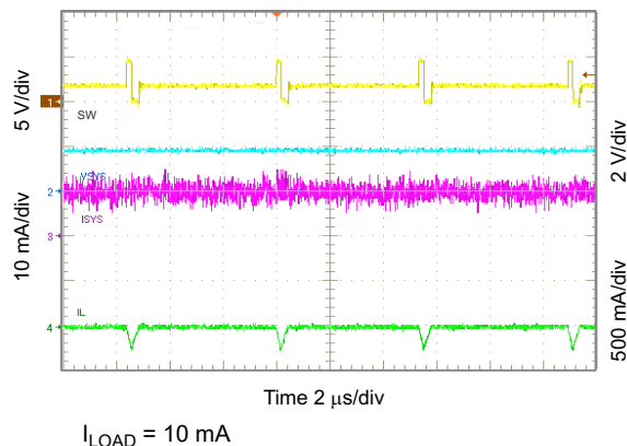
图 10-29. Light Load Operation Showing SW
