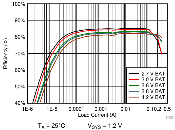
图 10-10. 1.2 V_{\text{SYS}} System Efficiency
