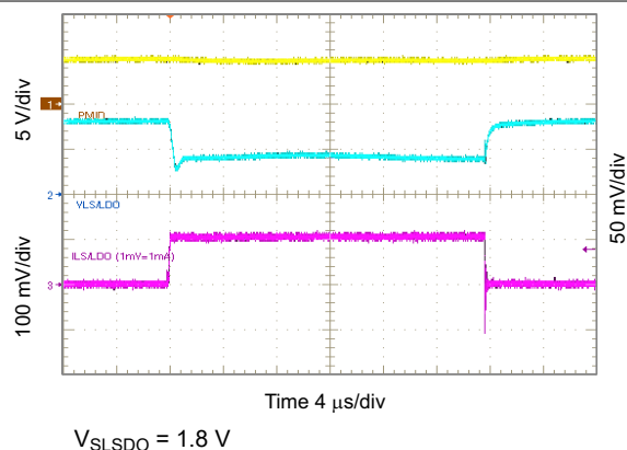
图 10-54. 1.8 V_{LSLDO} Load Transient, 0 to 100 mA
