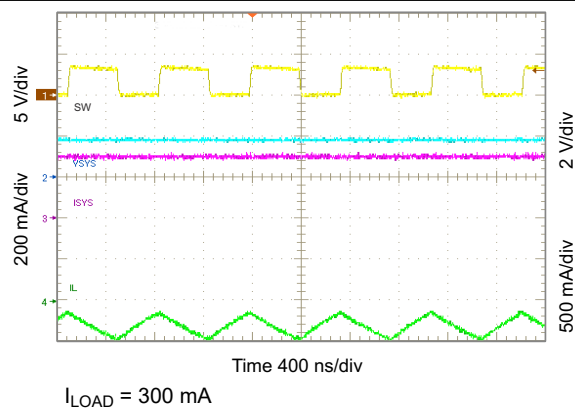
图 10-32. Light Load Operation Showing SW
