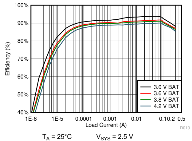
图 10-13. 2.5 V_{\text{SYS}} System Efficiency
