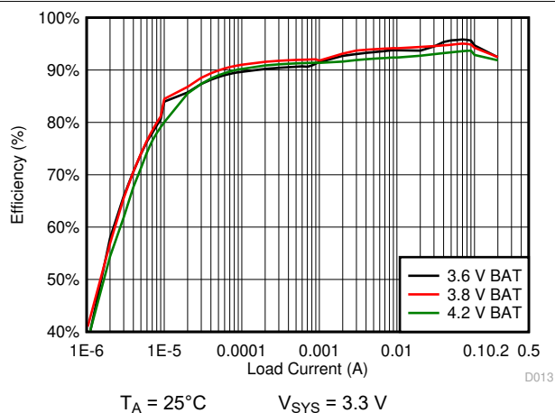
图 10-14. 3.3 V_{\text{SYS}} System Efficiency
