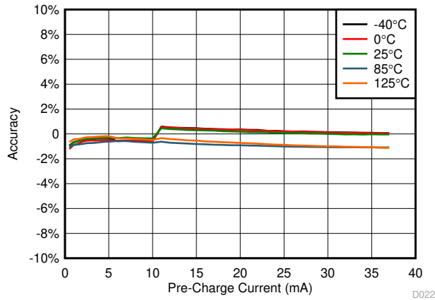
图 8-11. Pre-Charge Accuracy vs Pre-Charge Current
