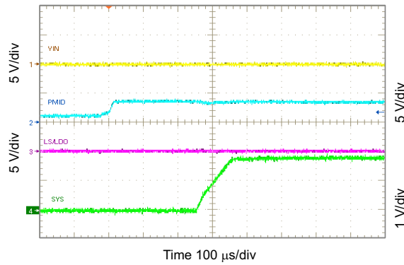
图 10-2. Battery Connected to V_{BAT}
