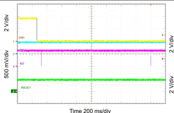
图 10-62. \overline{PG} Functions as Shifted \overline{MR} Output
