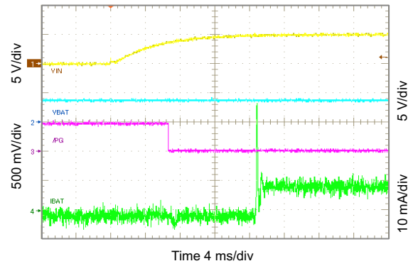
图 10-3. Power Supply Connected to V_{IN}
