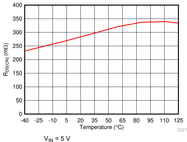
图 8-13. R_{DS(ON)} of Low Side MOSFET vs Temperature
