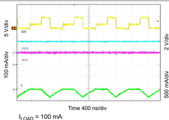
图 10-30. Light Load Operation Showing SW
