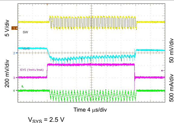
图 10-41. 2.5 V SYS Load Transient, 0 to 200 mA
