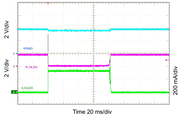
图 10-58. Short Circuit and Recovery for LDO
