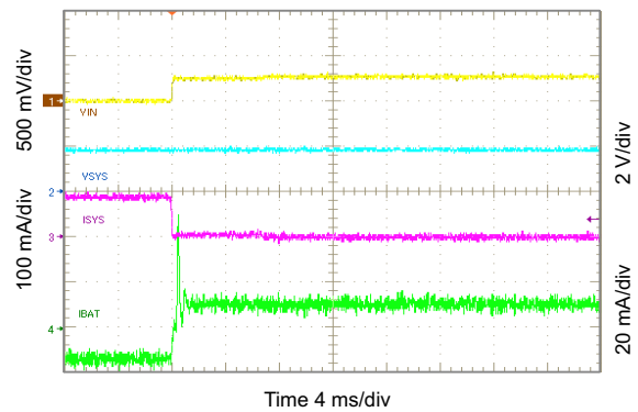
图 10-7. Exiting Battery Supplement Mode
