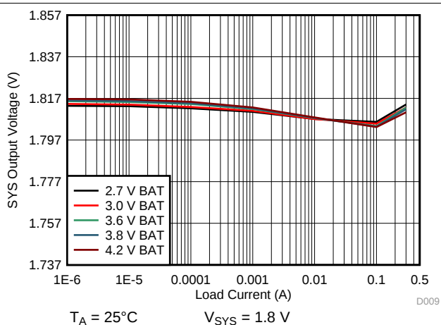
图 51. 1.8 V sys Load Regulation
