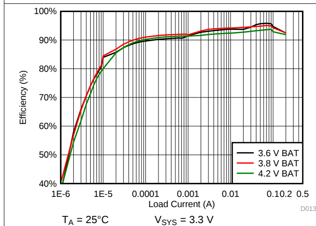
图 48. 3.3 V SYS System Efficiency
