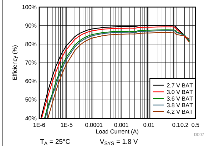
图 46. 1.8 V SYS System Efficiency
