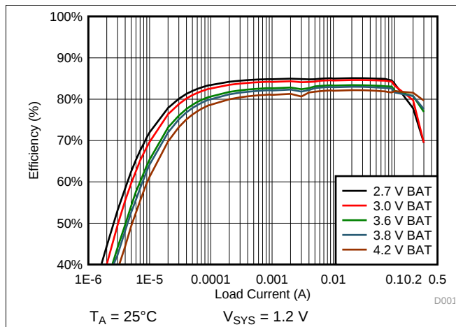
图 44. 1.2 V SYS System Efficiency
