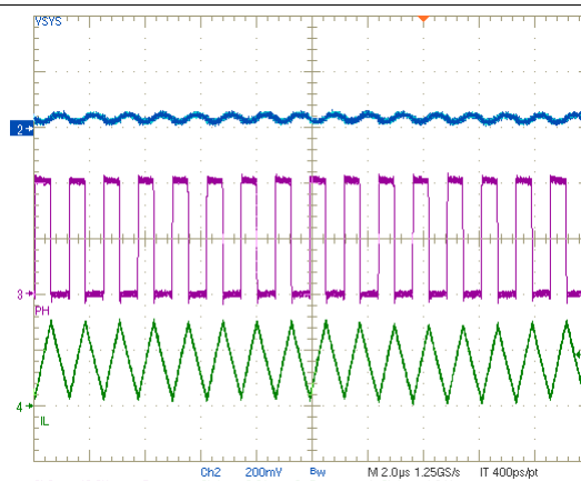
Figure 27. Current Disabled
