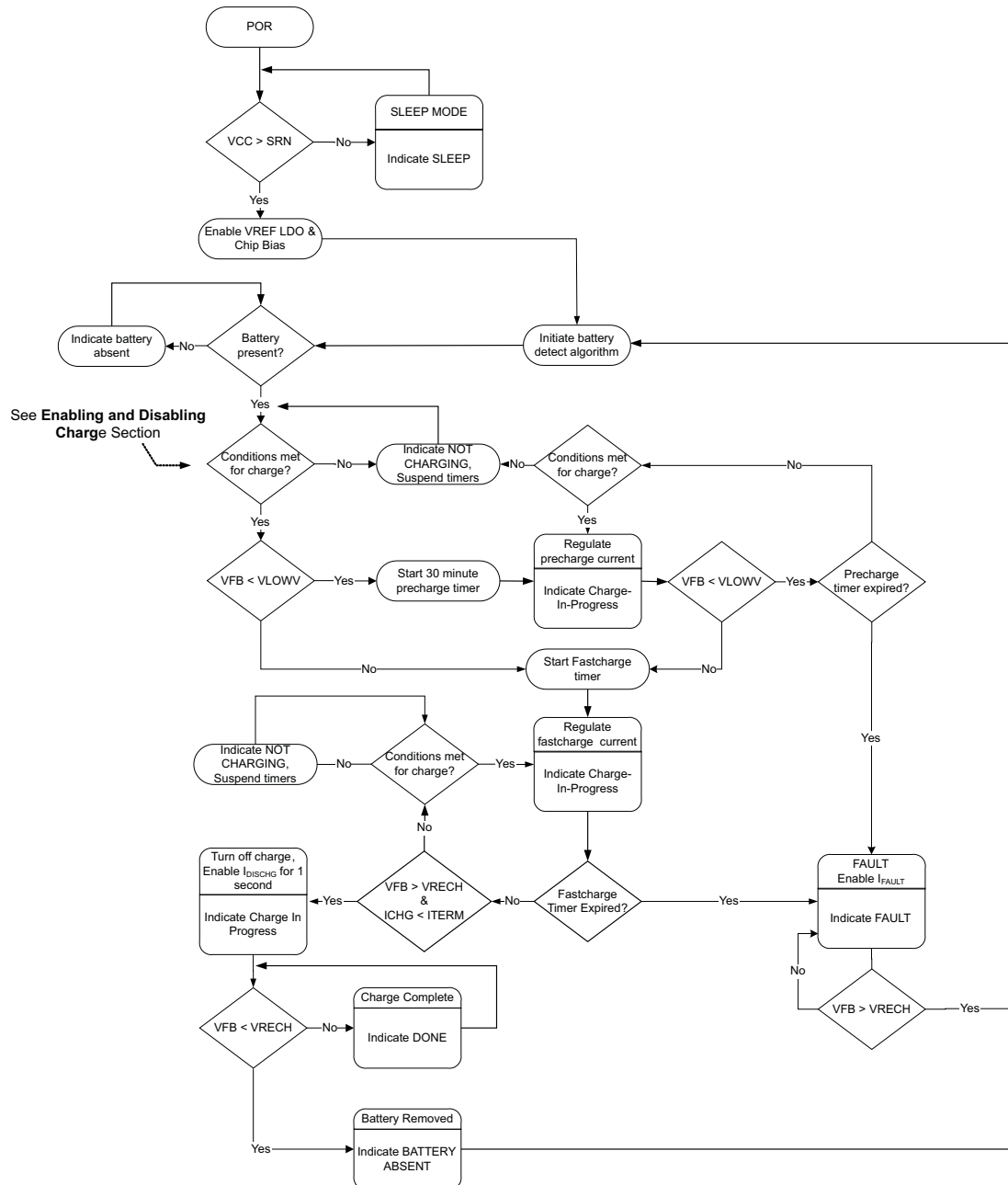
Figure 14. Operational Flowchart for BQ24650
