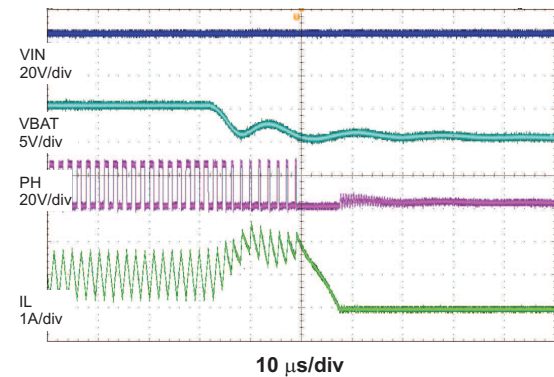
Figure 22. Charge Reset During Battery Short
