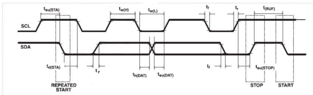
图 8-1. I²C-Compatible Interface Timing Diagram
