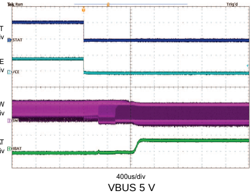
图 39. Power Up with Charge Disabled
