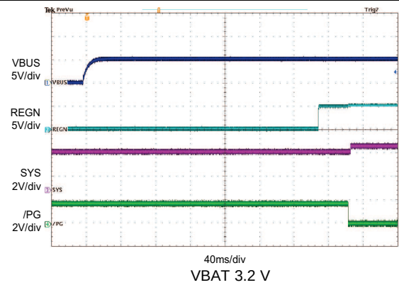
图 39. Power Up with Charge Disabled
