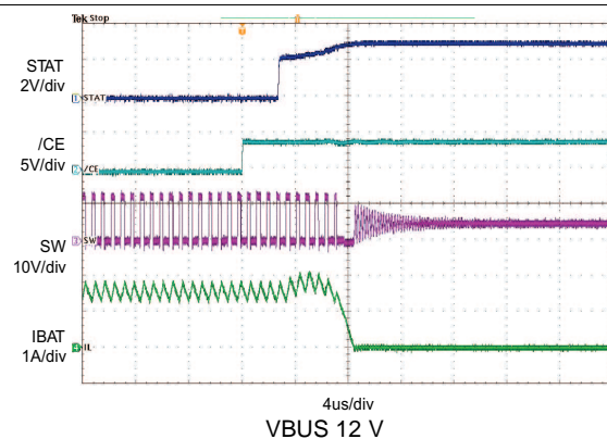
图 39. Power Up with Charge Enabled
