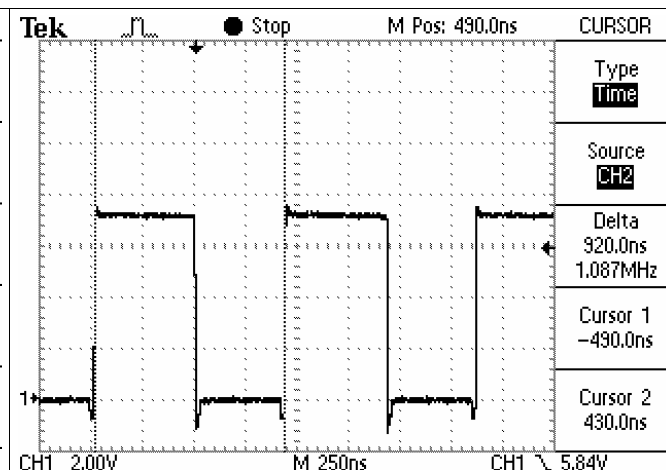
Figure 22. Fast Charge Waveform
