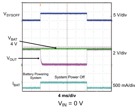
Figure 32. BQ24075T, BQ24079T System On/Off With Input Not Connected
