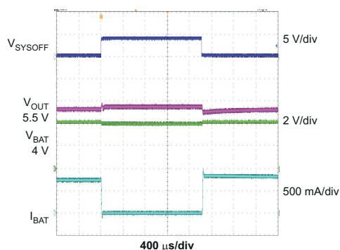
图 10-10. System ON/OFF With Input Connected V_{\text{IN}} = 6 \text{ V} BQ24075, BQ24079
