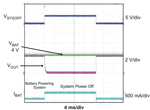
图 10-11. System ON/OFF With Input Not Connected V_{\text{IN}} = 0 \text{ V} BQ24075, BQ24079
