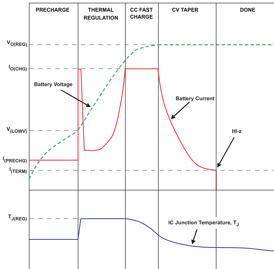
图 9-8. Charge Cycle Modified by Thermal Loop
