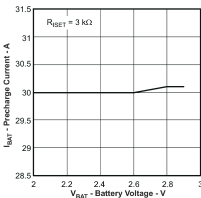
图 8-15. Precharge Current vs Battery Voltage
