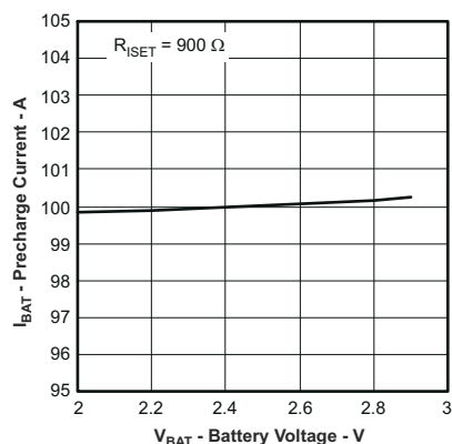
图 8-14. Precharge Current vs Battery Voltage
