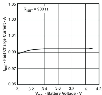
图 8-12. Fastcharge Current vs Battery Voltage
