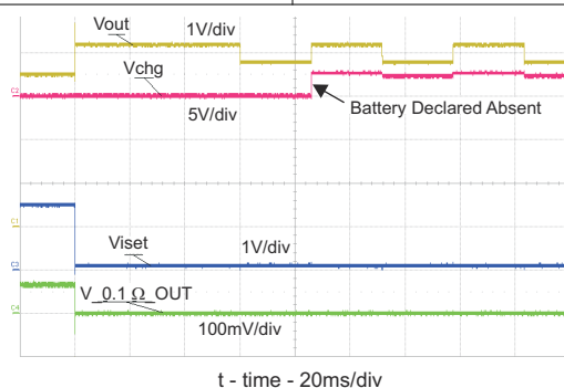
图 6-6. Battery Removal With OUT and TS Disconnect First
