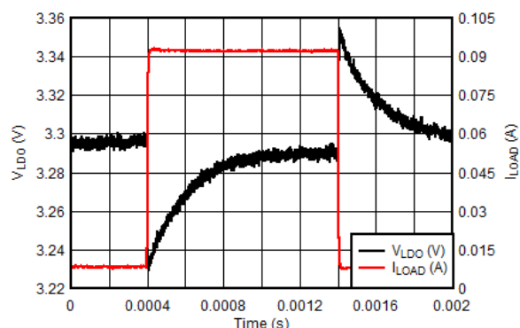
图 8-19. LDO Load Transient - VLDO = 3.3V
