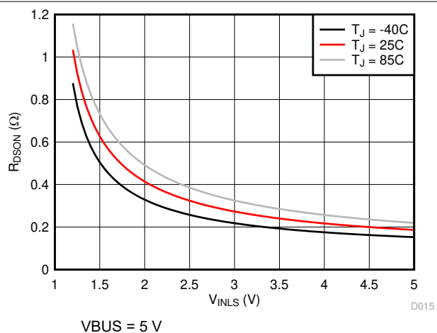
图 6-5. LS/LDO Switch On Resistance vs. VINLS
