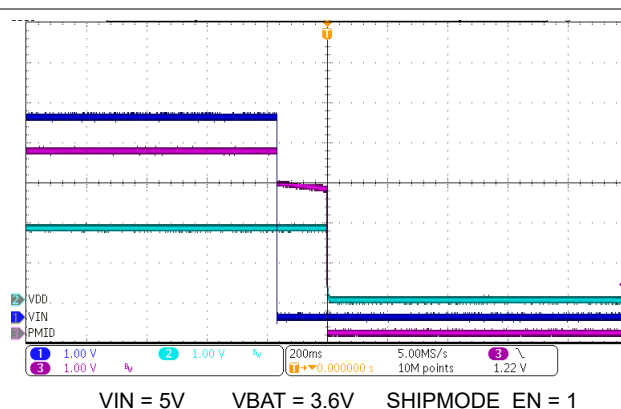
图 8-9. Ship Mode Entry on IN Supply Removal
