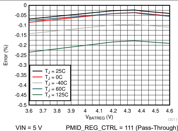
图 6-1. Battery Regulation Voltage Accuracy vs. VBATREG Setting
