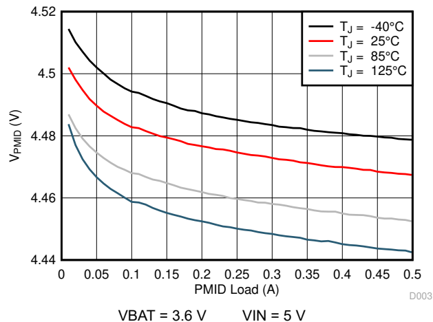
图 6-14. PMID Load Regulation vs. Temperature
