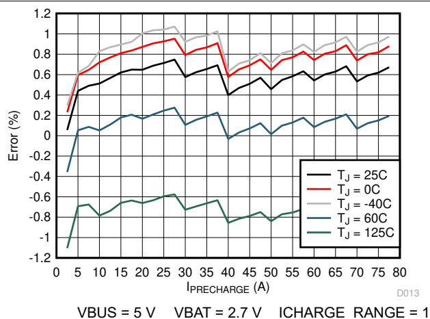
图 6-4. Pre-Charge Current Accuracy vs. IPRECHARGE Setting (ICHARGE_RANGE = 1)
