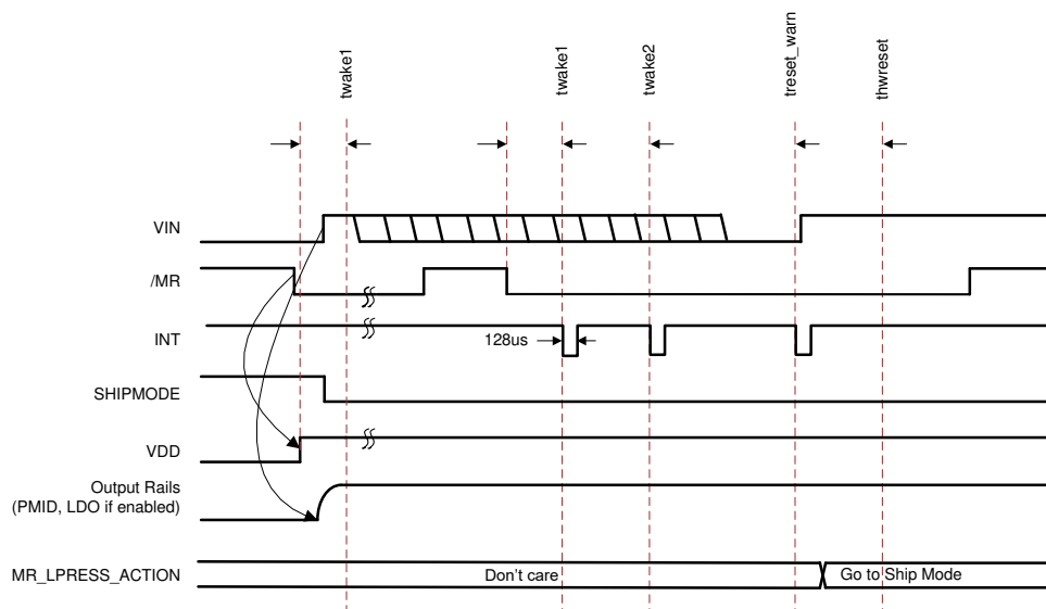
图 7-4. MR Wake from Ship Mode - V_{\text{IN}} Dependencies
