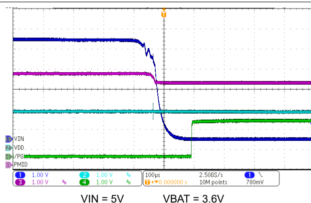
图 8-11. \overline{\text{PG}} Power Good Function - IN Supply Removal
