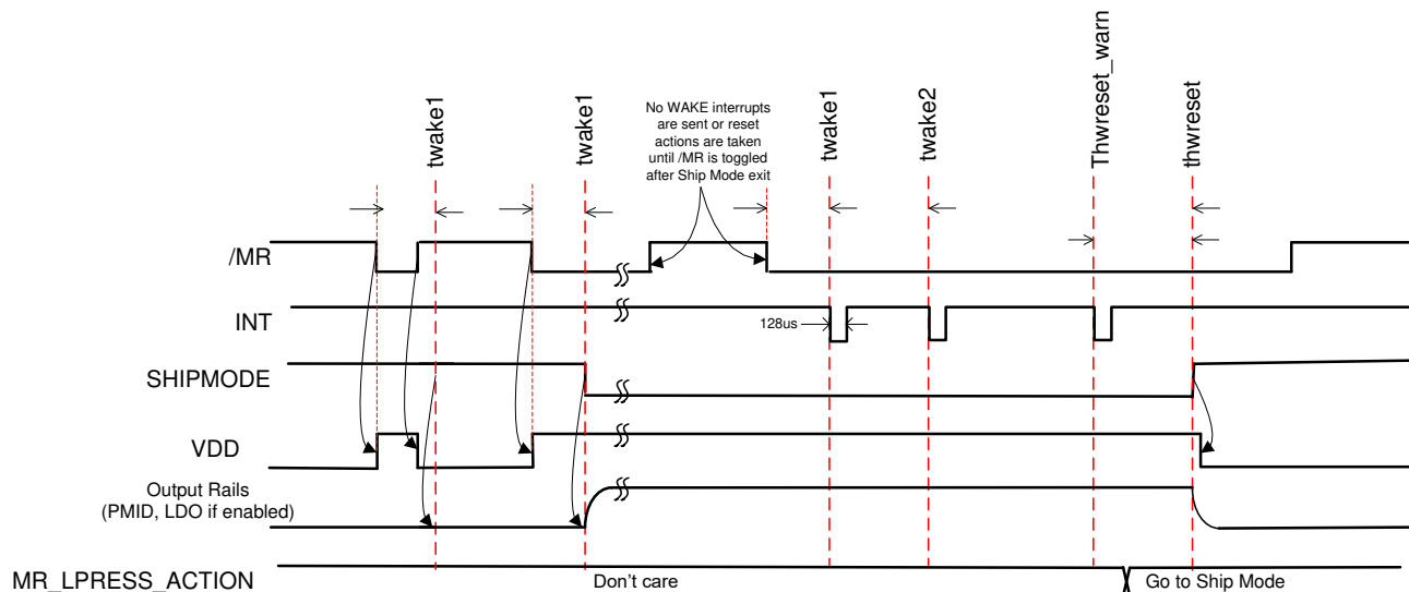
图 7-3. MR Wake from Ship Mode ( \text{MR\_LPRESS\_ACTION} = Ship Mode, V_{\text{IN}} not valid)
