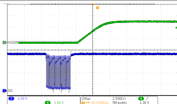
图 8-15. LDO Enable Through I²C (EN_LS_LDO)
