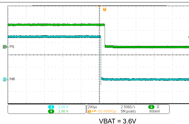
图 8-13. \overline{\text{PG}} \overline{\text{MR}} Level Shift Function - \overline{\text{MR}} Falling
