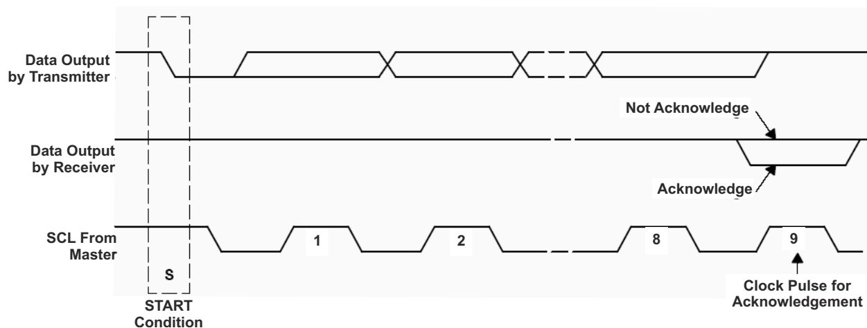
图 7-11. Acknowledge on the I 2 C Bus
