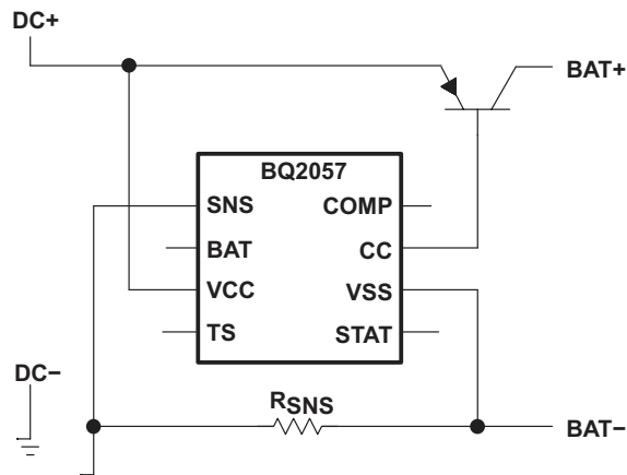
图 10-6. Low-Side Current Sensing
