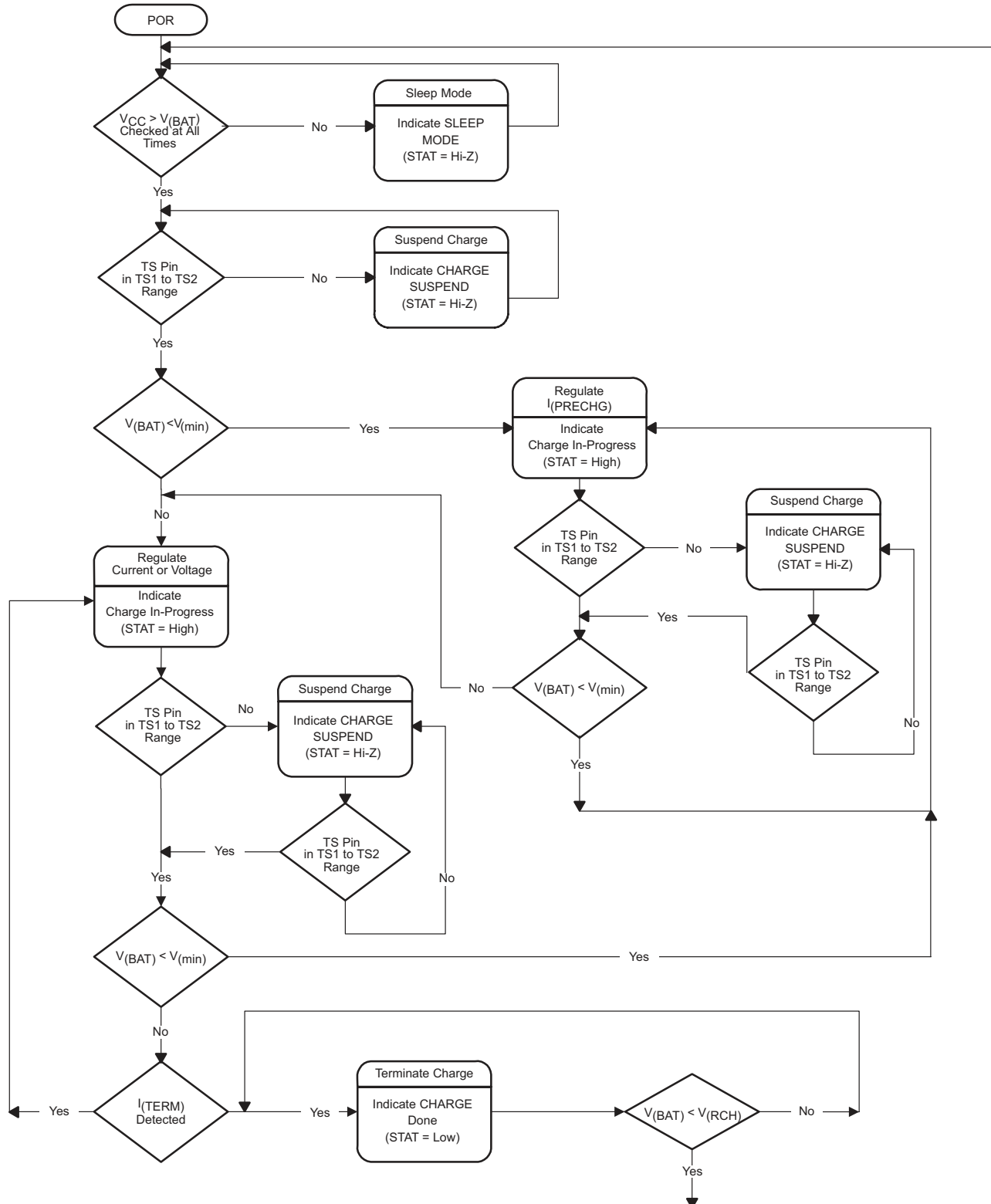
图 10-2. Operation Flowchart
