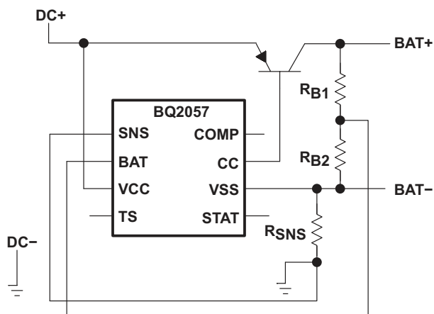
图 10-8. Optional Voltage Divider for Nonstandard Regulation Voltage, (Low-Side Current Sensing)
