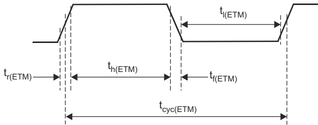
图 7-26. ETMTRACECLKOUT 时序
