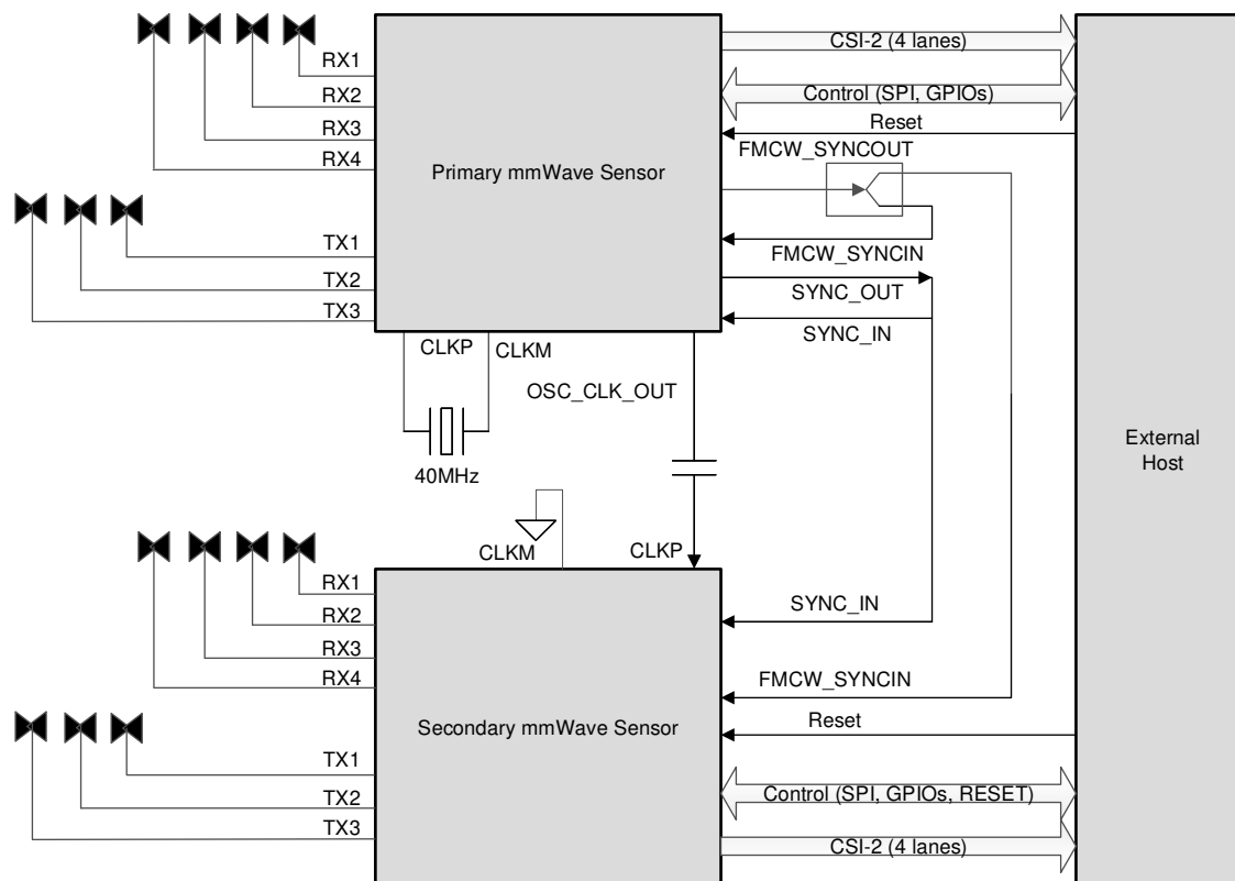
图 10-2. Imaging Radar using Cascade Configuration
