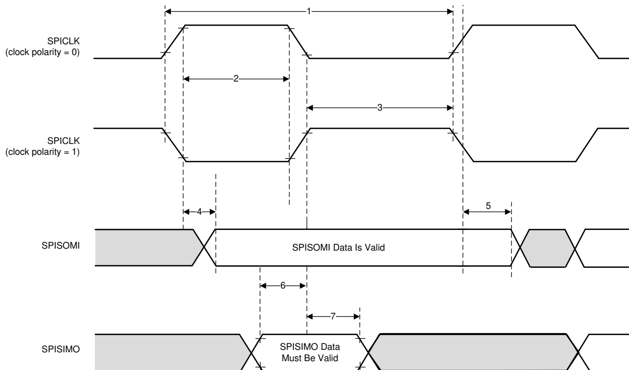
图 6-12. SPI Peripheral Mode External Timing (CLOCK PHASE = 0)
