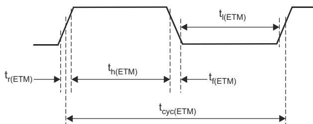
图 6-20. ETMTRACECLKOUT Timing
