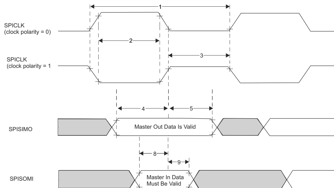
图 6-8. SPI Controller Mode External Timing (CLOCK PHASE = 0)
