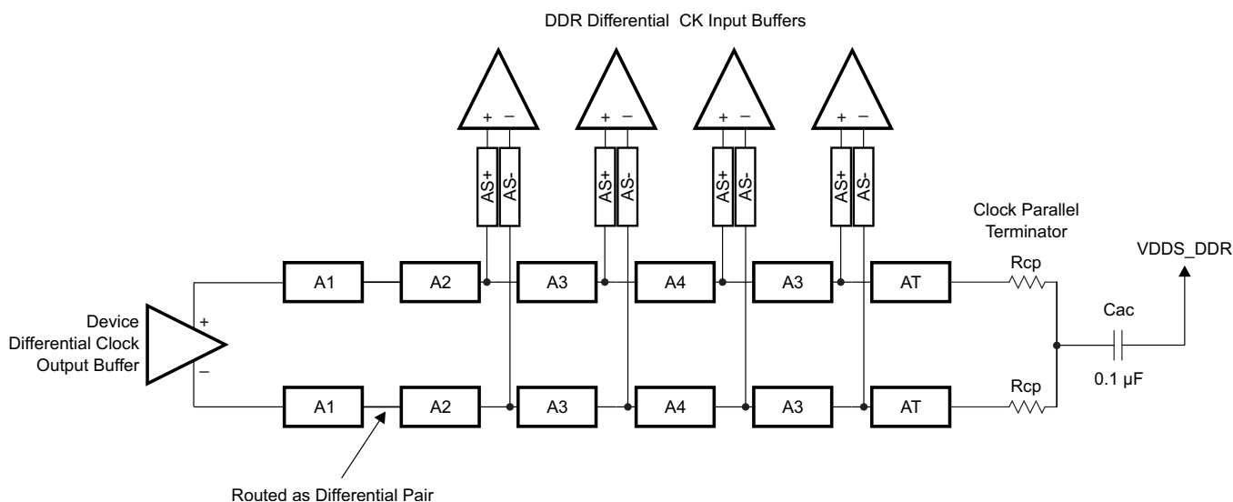
图 5-62. CK Topology for Four DDR3 Devices
