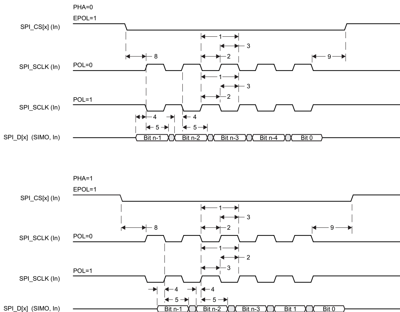
图 7-73. SPI Slave Mode Receive Timing
