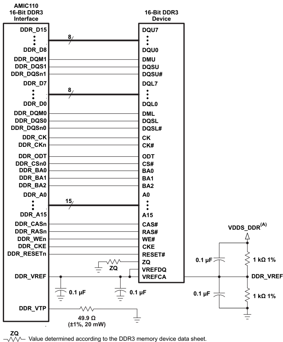
图 7-48. 16-Bit DDR3 Interface Using One 16-Bit DDR3 Device without V TT Termination
