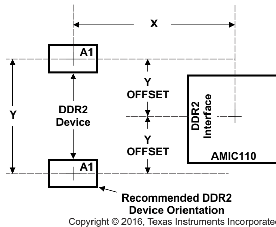
图 7-41. AMIC110 Device and DDR2 Device Placement
