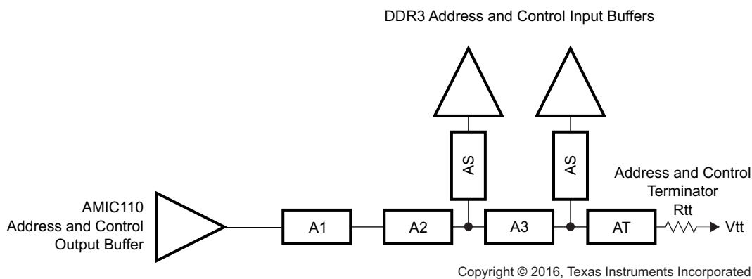
图 7-53. ADDR_CTRL Topology for Two DDR3 Devices
