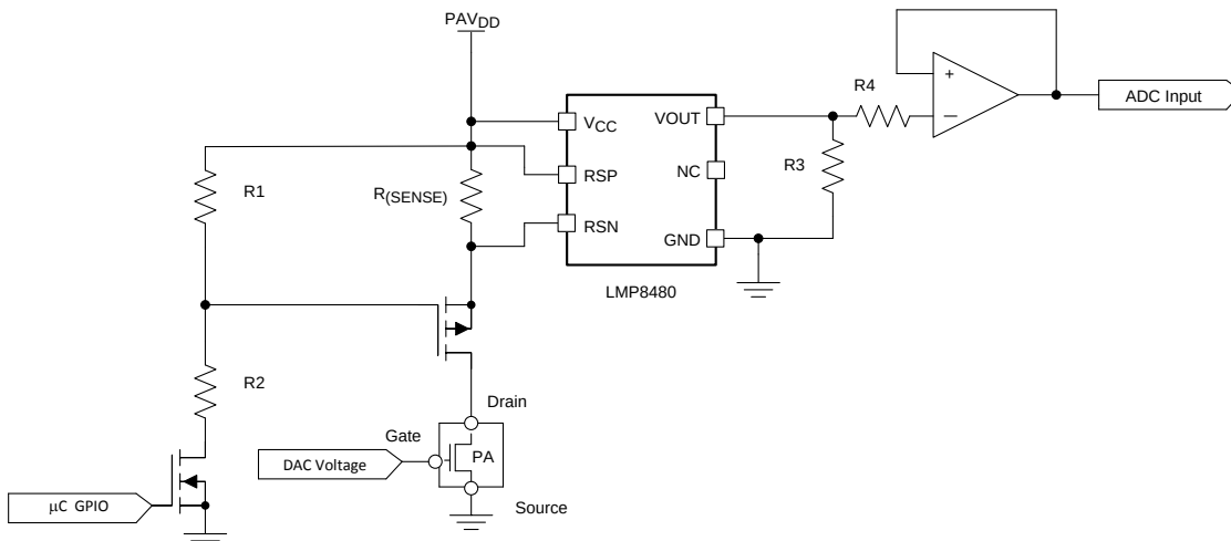
图 117. Current-Sense Application With PMOS ON and OFF
