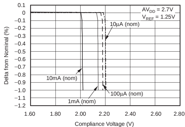
PRECISION I OUT vs COMPLIANCE VOLTAGE
