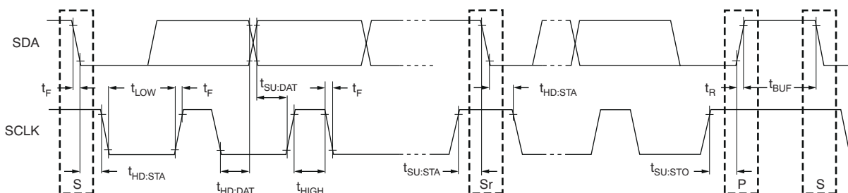
图 7-1. Timing Specification
