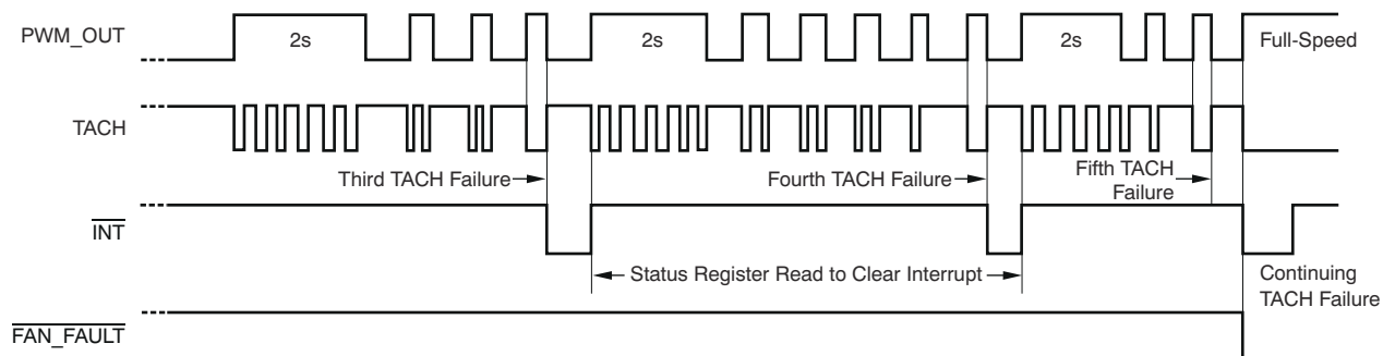
图 8-10. Operation of the \overline{\text{FAN-FAULT}} Pin With a Spin-Up Time = 2 Seconds
