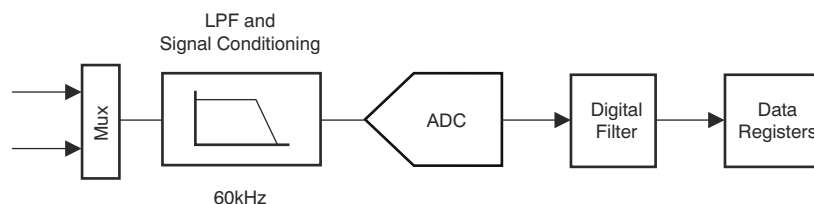
图 8-1. On-Chip Analog-to-Digital Converter
