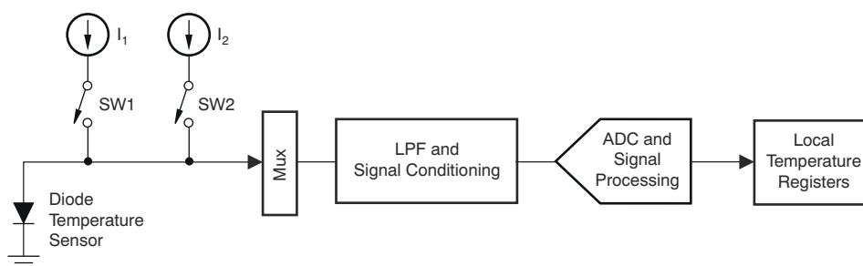
图 8-2. Integrated Local Temperature Sensor
