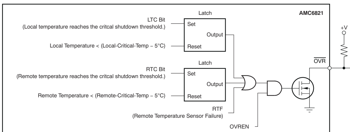
图 8-20. \overline{\text{OVR}} Pin
