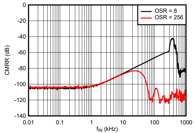
图 6-37. Common-Mode Rejection Ratio vs Input Signal Frequency
