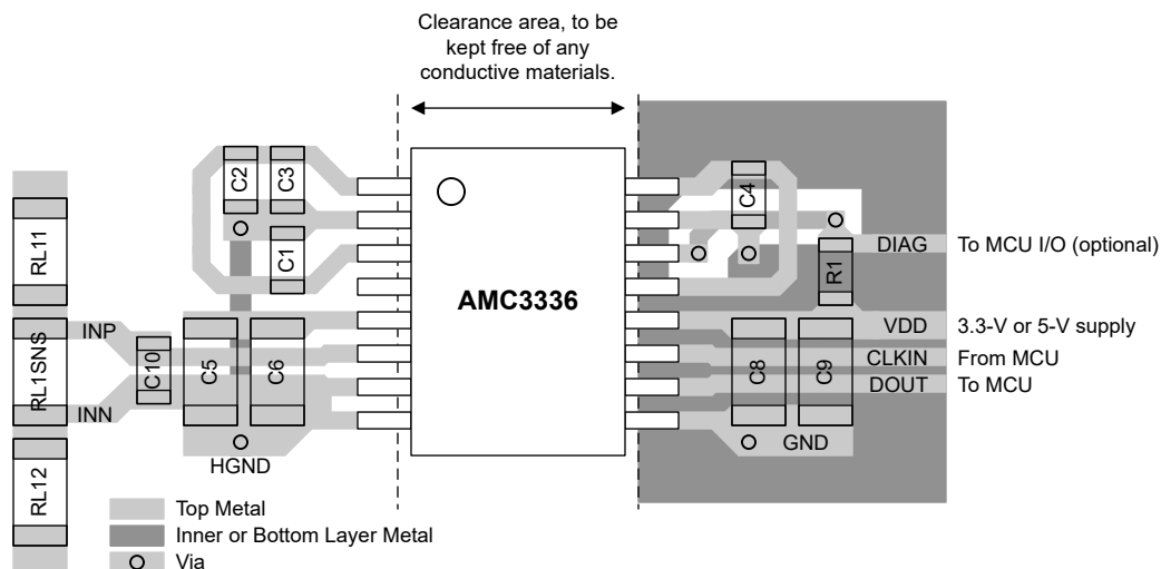
图 10-1. Recommended Layout of the AMC3336
