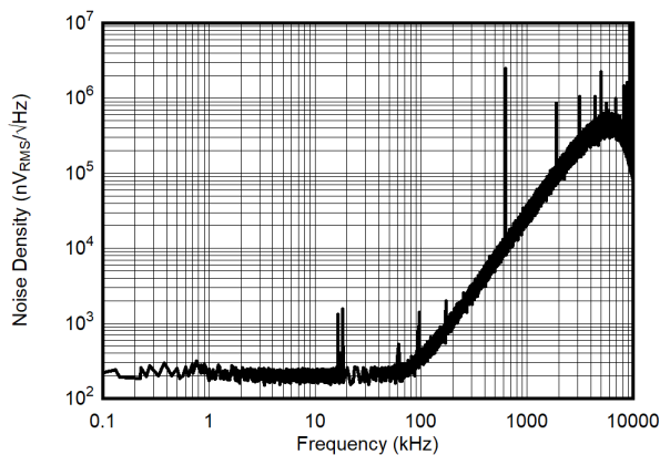
图 6-34. Noise Density With Both Inputs Shorted to HGND
