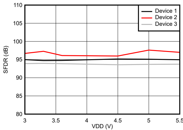
图 6-32. Spurious-Free Dynamic Range vs Supply Voltage
