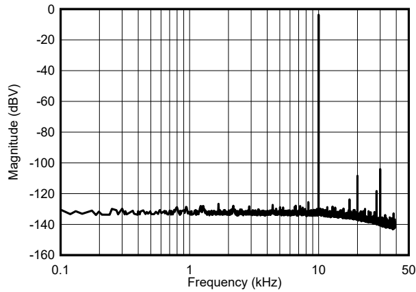
图 6-36. Frequency Spectrum With 10-kHz Input Signal
