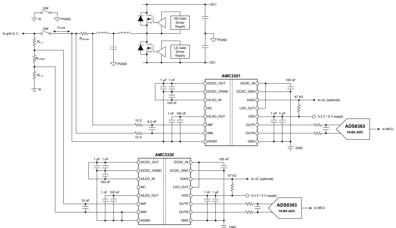
图 7-1. The AMC3330 in a Solar Inverter Application
