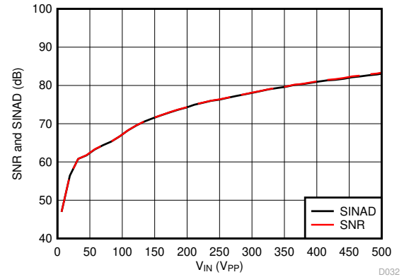
图 6-19. Signal-to-Noise Ratio and Signal-to-Noise + Distortion vs Input Signal Amplitude
