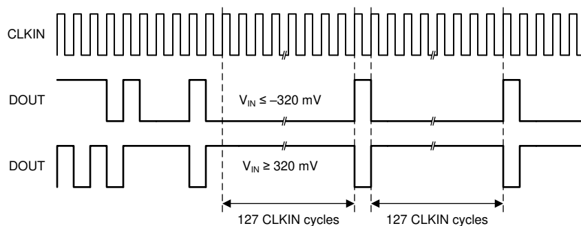
图 7-5. Full-Scale Output of the AMC3306M25
