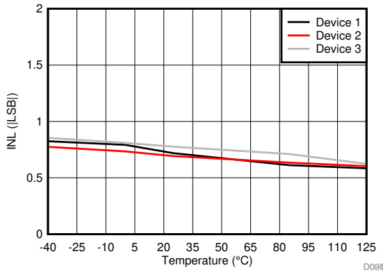
图 6-18. Integral Nonlinearity vs Temperature
