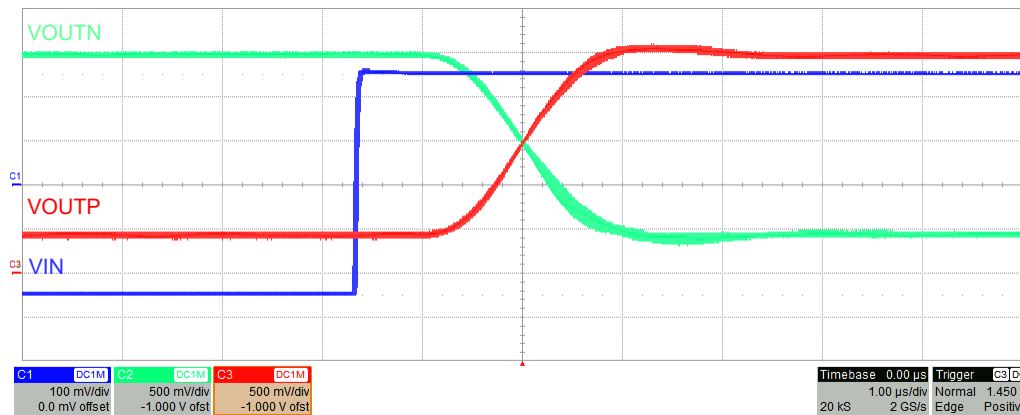
图 8-4. Step Response of the AMC1400-Q1
