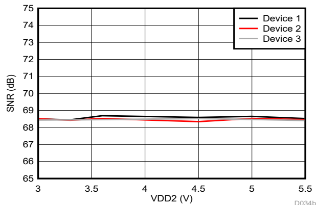
图 6-24. Signal-to-Noise Ratio vs Low-Side Supply Voltage
