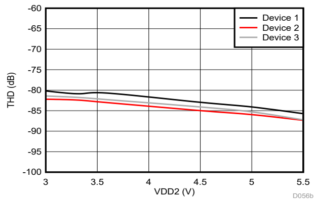
图 6-18. Total Harmonic Distortion vs Input Voltage
