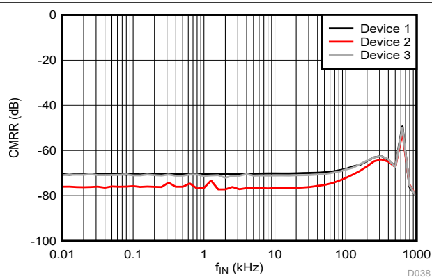
图 6-28. Common-Mode Rejection Ratio vs Input Frequency
