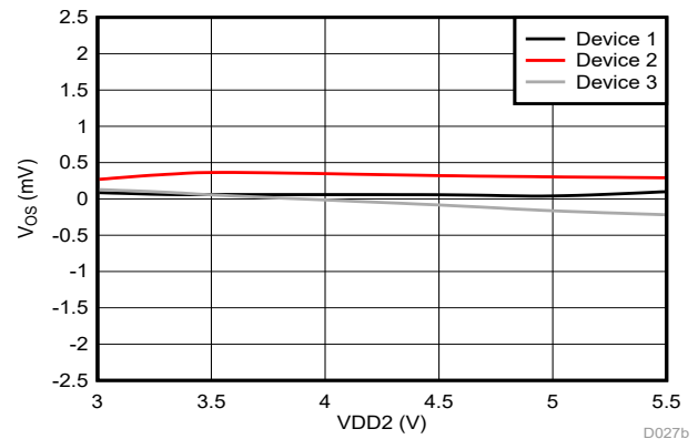
图 6-8. Input Offset Voltage vs Low-Side Supply Voltage
