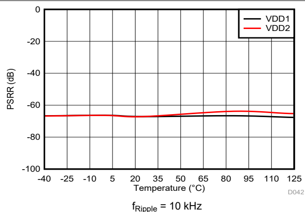
图 6-32. Power-Supply Rejection Ratio vs Temperature
