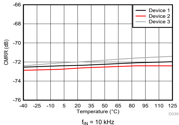
图 6-30. Common-Mode Rejection Ratio vs Temperature
