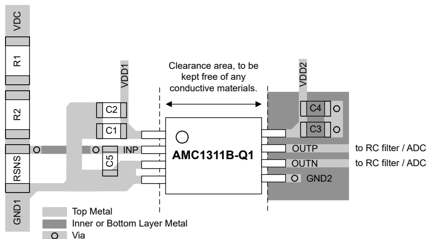
Figure 10-1. Recommended Layout of the AMC1311-Q1
