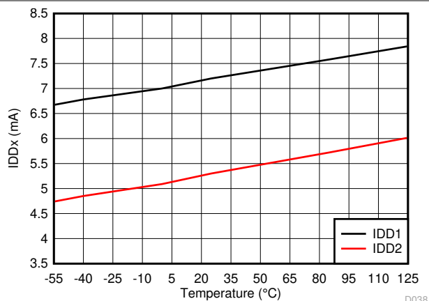
图 7-36. Supply Current vs Temperature
