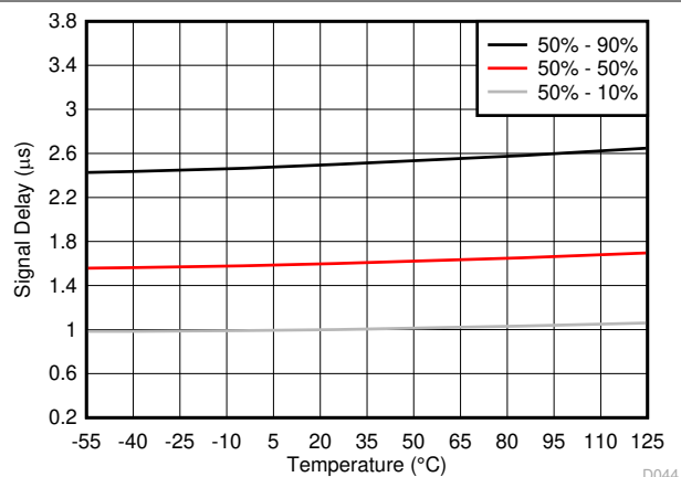
图 7-42. V_{IN} to V_{OUT} Signal Delay vs Temperature
