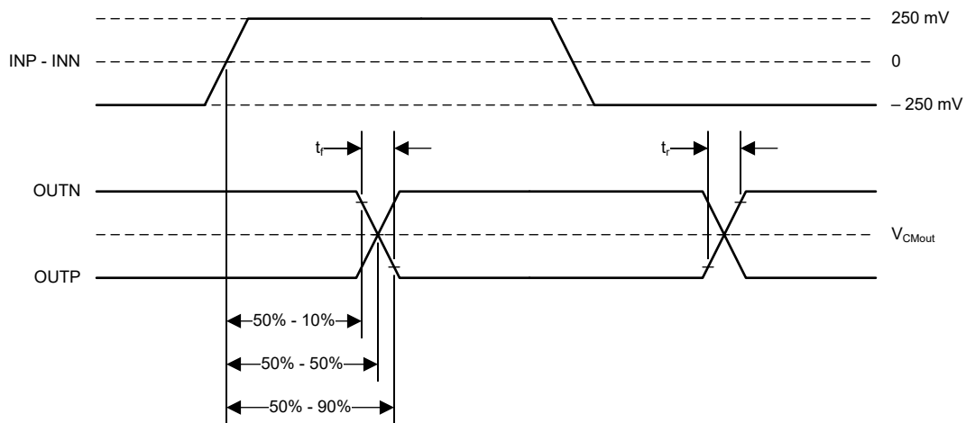
图 7-1. Rise, Fall, and Delay Time Waveforms
