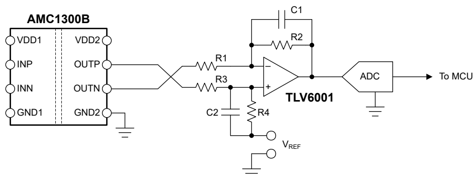
图 9-3. Connecting the AMC1300 Output to a Single-Ended Input ADC
