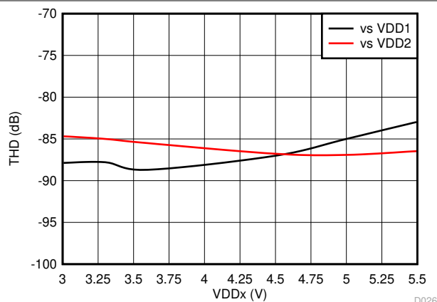
图 7-24. Total Harmonic Distortion vs Supply Voltage
