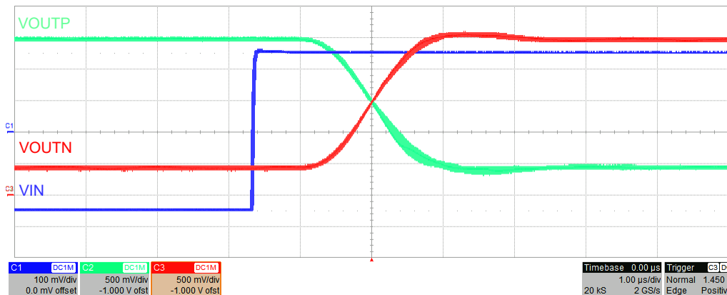
图 9-4. Step Response of the AMC1300
