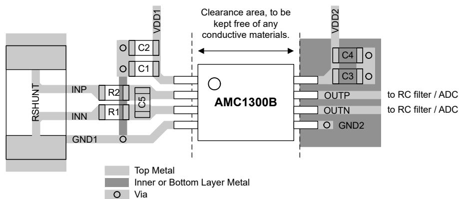
图 11-1. Recommended Layout of the AMC1300
