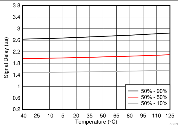
图 7-41. V_{IN} to V_{OUT} Signal Delay vs Temperature
