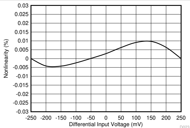
图 7-21. Nonlinearity vs Input Voltage
