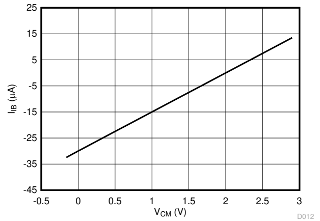
图 7-12. Input Bias Current vs Common-Mode Input Voltage
