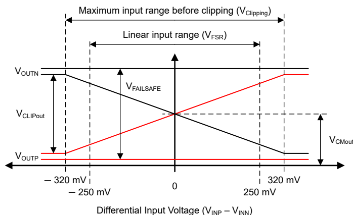
图 8-2. Output Behavior of the AMC1300
