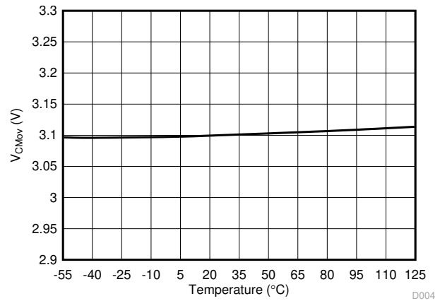
图 7-6. Common-Mode Overvoltage Detection Level vs Temperature
