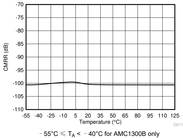
图 7-11. Common-Mode Rejection Ratio vs Temperature
