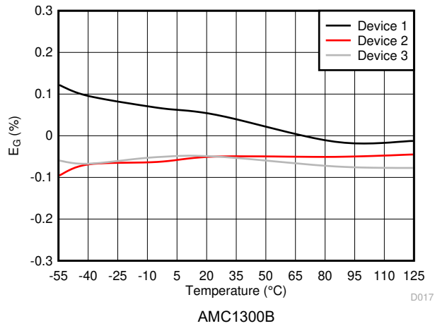
图 7-17. Gain Error vs Temperature
