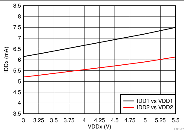
图 7-35. Supply Current vs Supply Voltage
