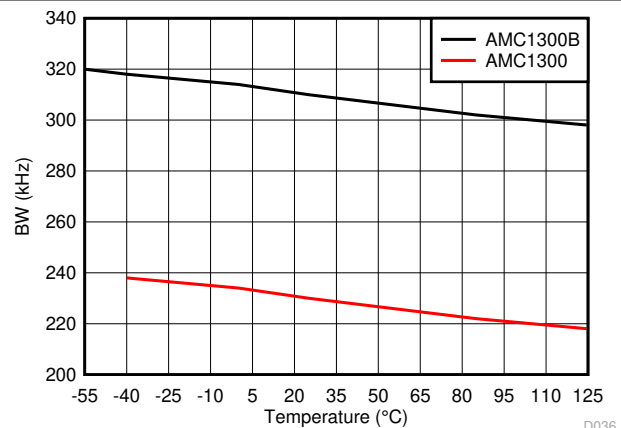
图 7-34. Output Bandwidth vs Temperature
