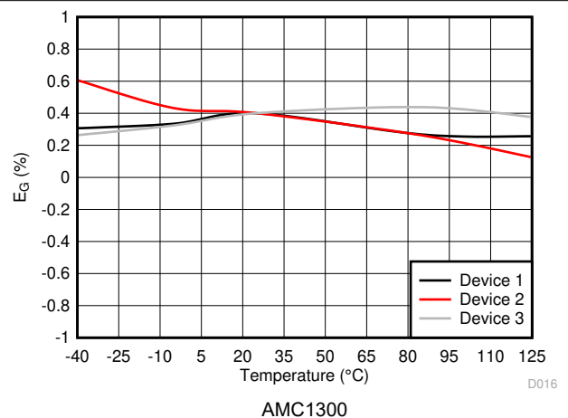
图 7-16. Gain Error vs Temperature
