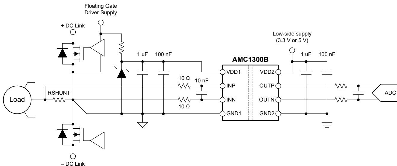
图 9-1. Using the AMC1300 for Current Sensing in a Typical Application
