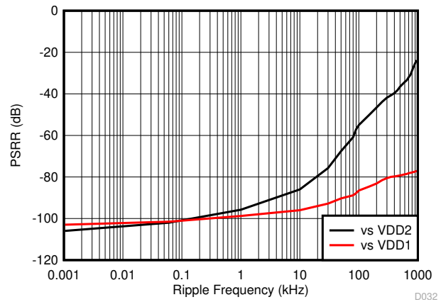
图 7-30. Power-Supply Rejection Ratio vs Ripple Frequency
