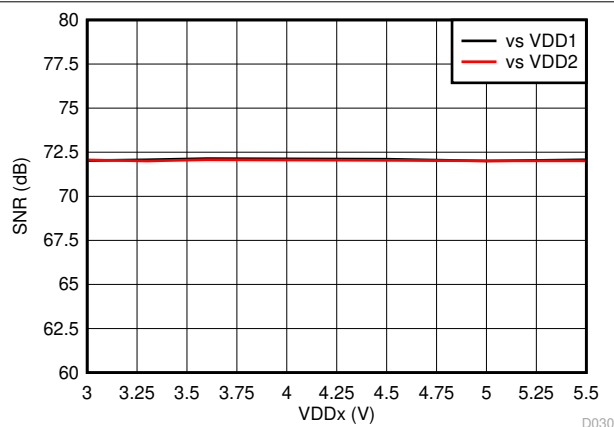
图 7-28. Signal-to-Noise Ratio vs Supply Voltage
