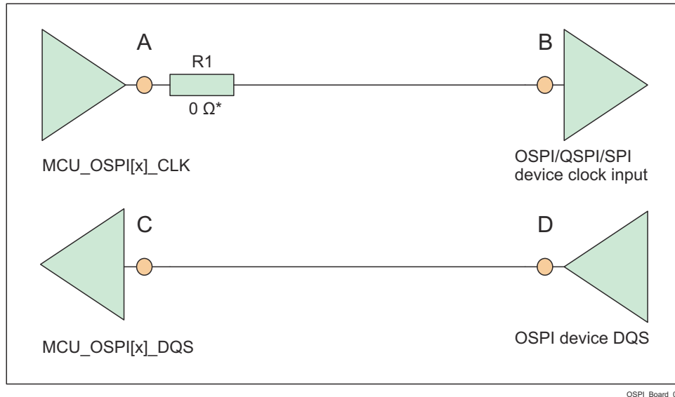
图 8-3. OSPI Interface High Level Schematic
