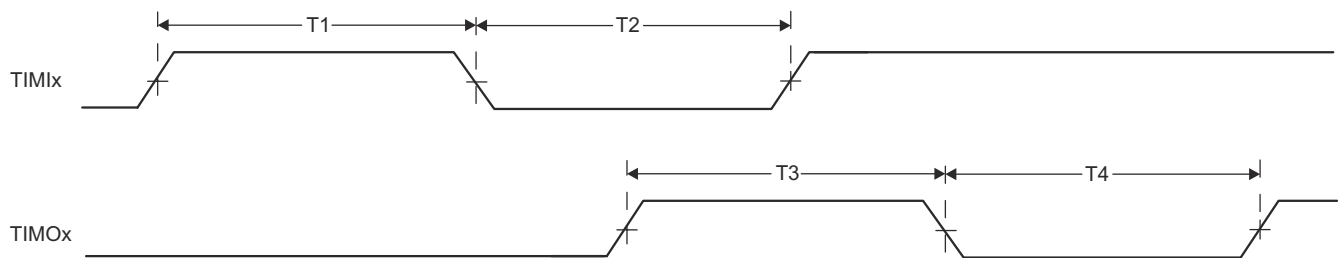
图 6-122. Timer Timing
