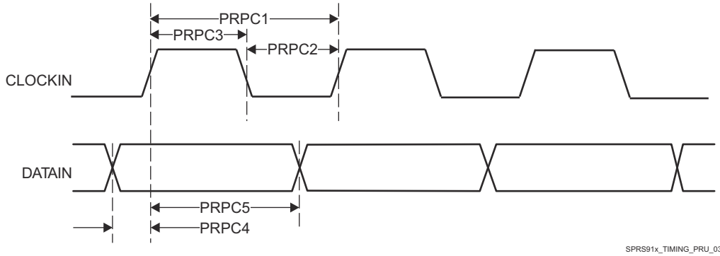
图 6-96. PRU_ICSSG PRU Parallel Capture Timing - Rising Edge Mode
