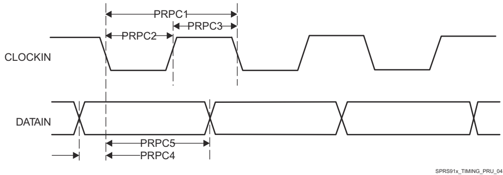
图 6-97. PRU_ICSSG PRU Parallel Capture Timing - Falling Edge Mode
