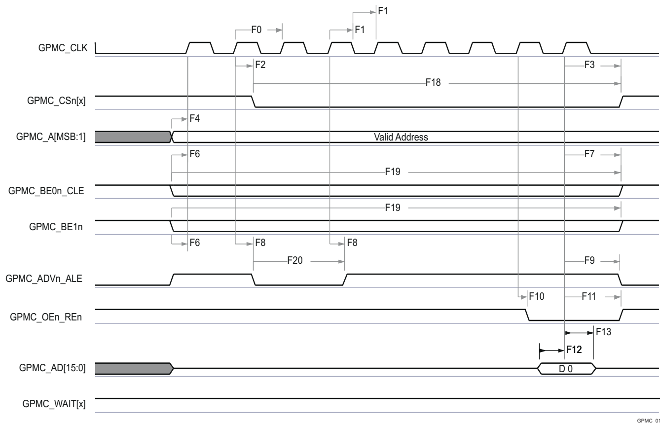
图 6-48. GPMC and NOR Flash—Synchronous Single Read—(GpmcFCLKDivider = 0)
