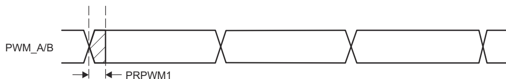
图 6-104. PRU_ICSSG PRU PWM Timing
