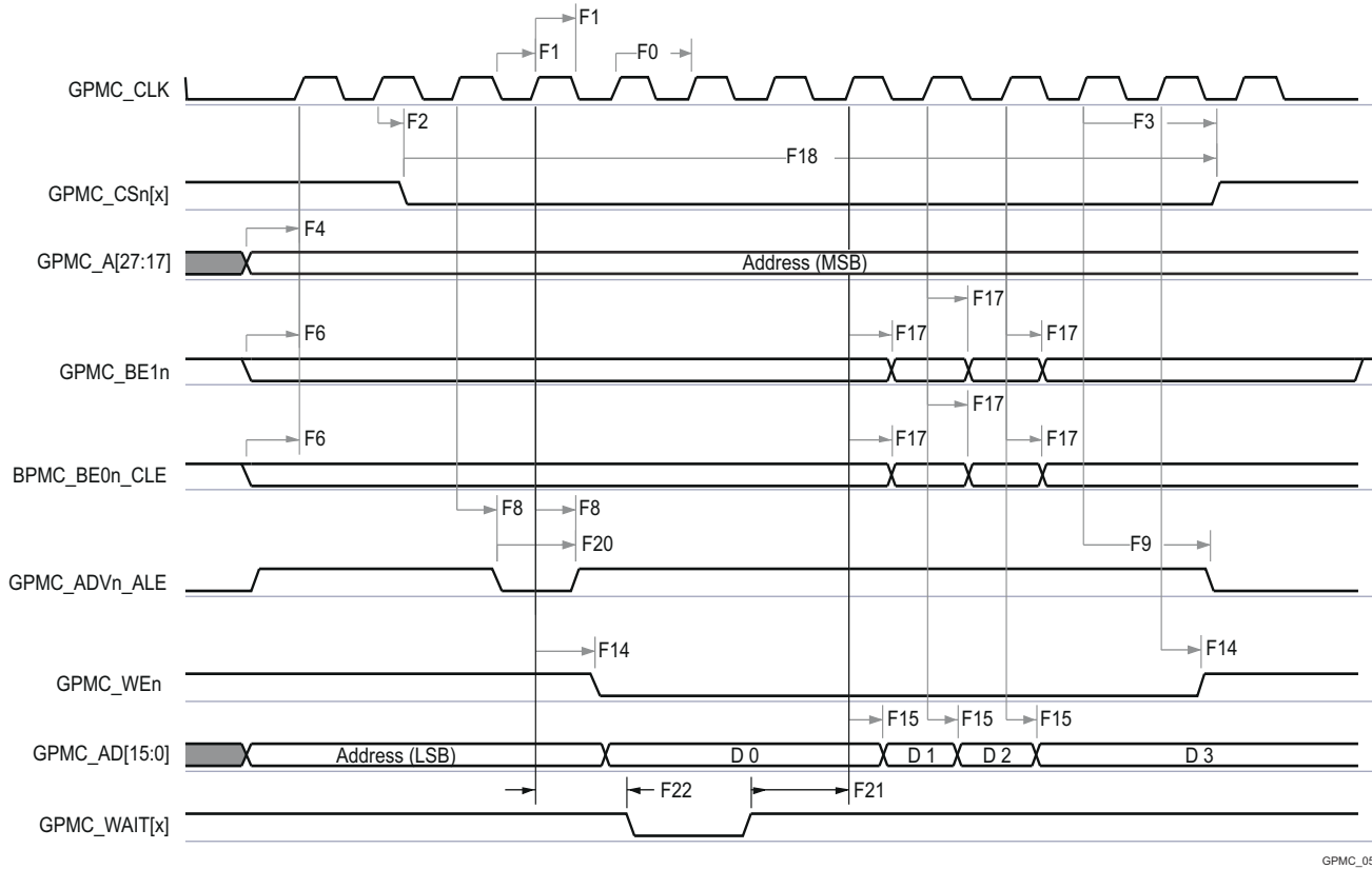
图 6-51. GPMC and Multiplexed NOR Flash—Synchronous Burst Read
