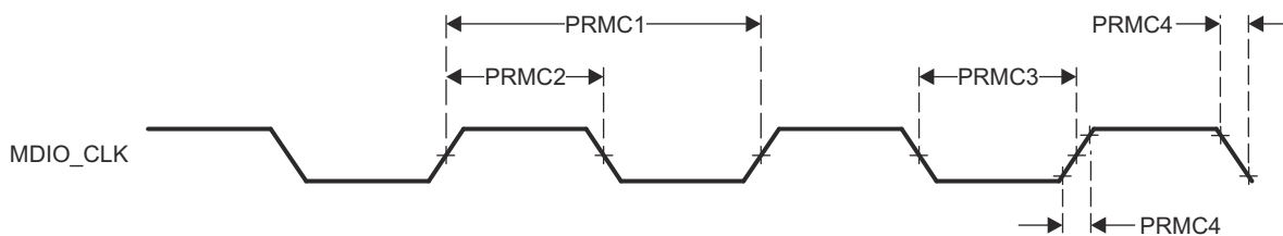
图 6-112. PRU_ICSSG MDIO_CLK Switching Characteristics
