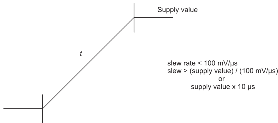
图 6-2. Power Supply Slew and Slew Rate
