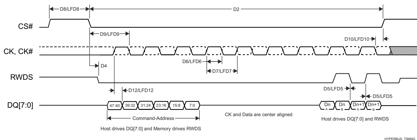
图 6-64. HyperBus Timing Diagrams - Receiver Mode
