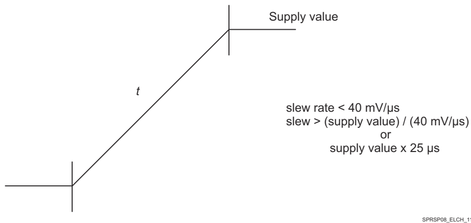
图 6-3. VDDA_1P8_SERDES0 Supply Slew and Slew Rate
