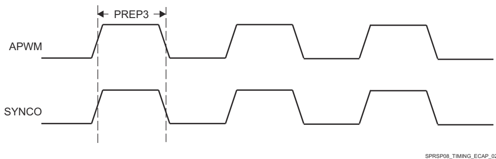
图 6-110. PRU_ICSSG ECAP Switching Characteristics
