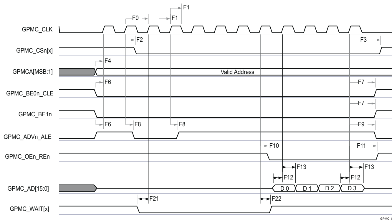
图 6-49. GPMC and NOR Flash—Synchronous Burst Read—4x16-bit (GpmcFCLKDivider = 0)
