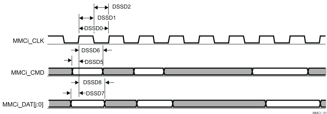
图 6-72. eMMC/SD/SDIO in - Default Speed - Receiver Mode
