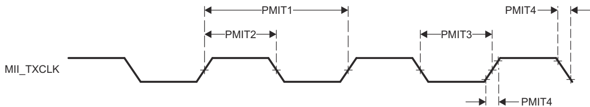
图 6-120. PRU_ICSSG MII_TX_CLK Switching Characteristics
