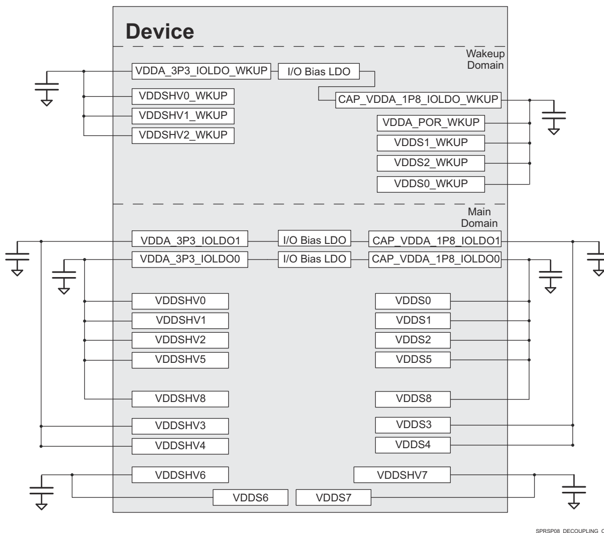
图 8-7. All VDDSHV[8:0], and VDDSHV[2:0]_WKUP Supplies Configured for 3.3 V Operation
