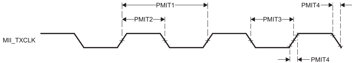
Figure 5-124. PRU-ICSS MII[x]_TXCLK Timing
