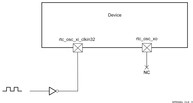
Figure 5-18. LVCMOS-Compatible Clock Input
