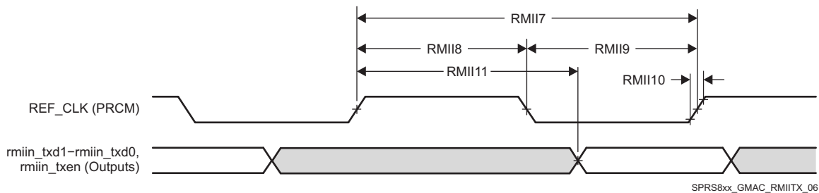
图 7-57. GMAC Transmit Interface Timing RMIIIn Operation
