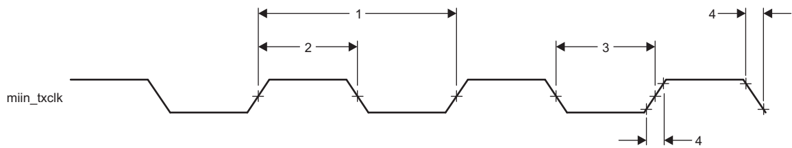
图 7-52. Clock Timing (GMAC Transmit) - MII operation
