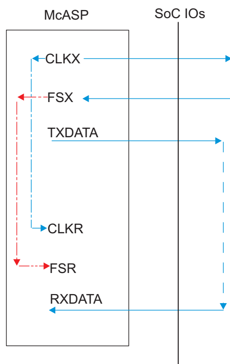
图 7-50. McASP1-8 CO-FI- – SYNC Mode
