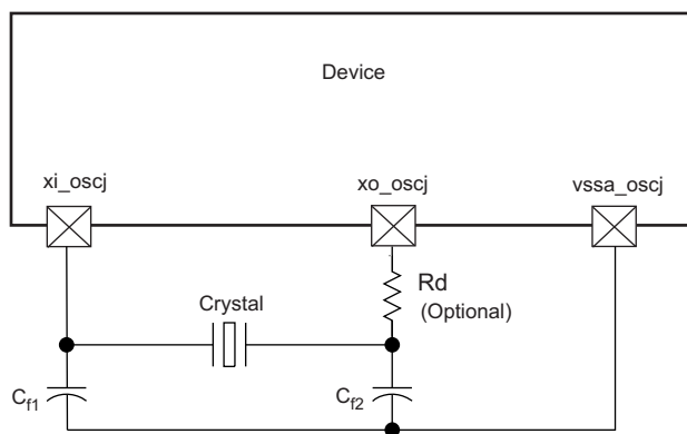
图 8-33. Grounding Scheme for High-Frequency Clock
