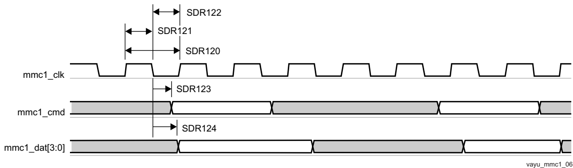
图 7-65. MMC/SD/SDIO in - High Speed SDR12 - Transmitter Mode
