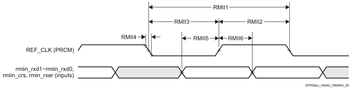
图 7-56. GMAC Receive Interface Timing RMIIIn operation
