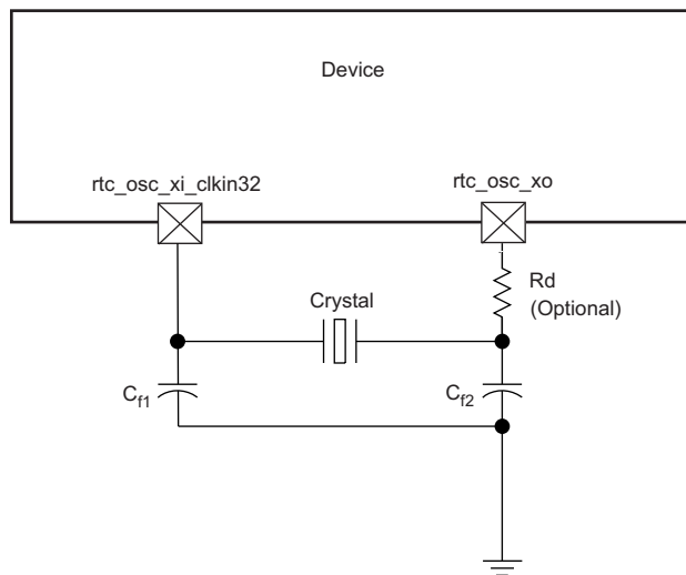
图 8-32. Grounding Scheme for Low-Frequency Clock
