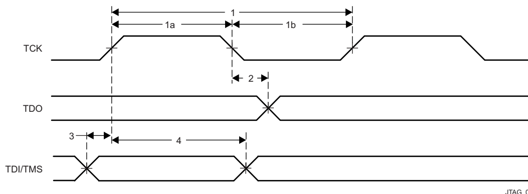
图 7-109. JTAG Timing
