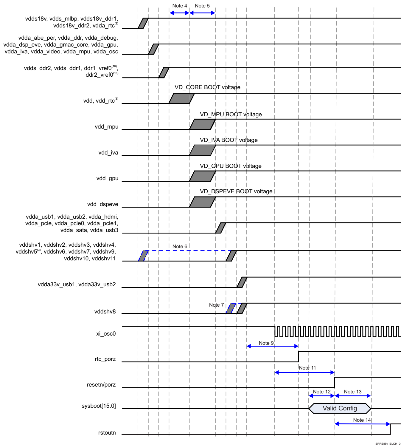
图 5-2. Power-Up Sequencing
