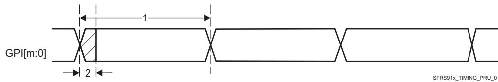
图 7-91. PRU-ICSS PRU Direct Input Timing
