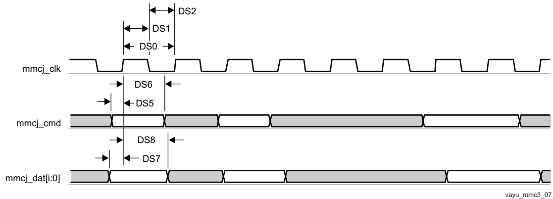
图 7-81. MMC/SD/SDIOj in - Default Speed - Receiver Mode
