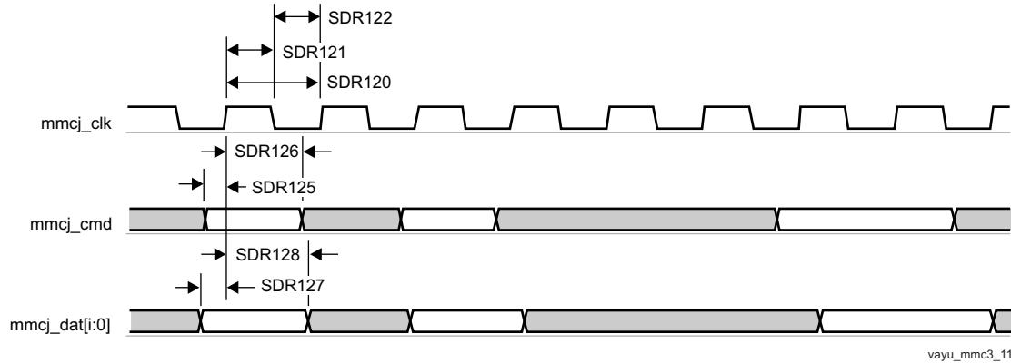
图 7-85. MMC/SD/SDIOj in - SDR12 - Receiver Mode
