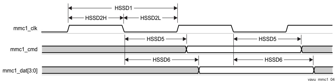
图 7-63. MMC/SD/SDIO in - High Speed - Transmitter Mode
