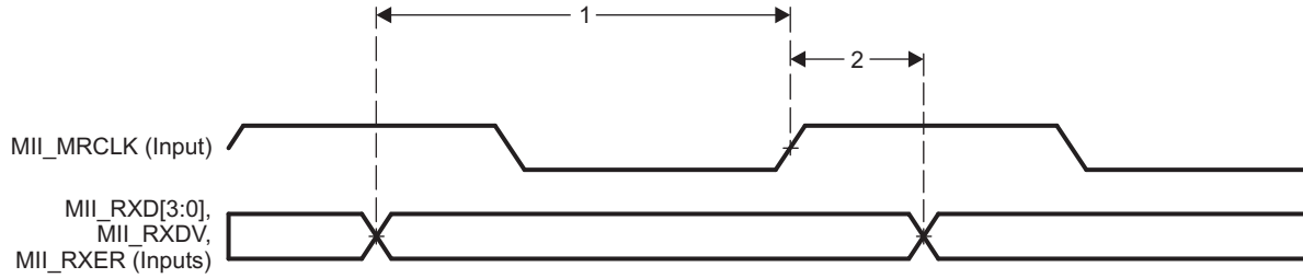
图 7-106. PRU-ICSS MII_RXD[3:0], MII_RXDV, and MII_RXER Timing
