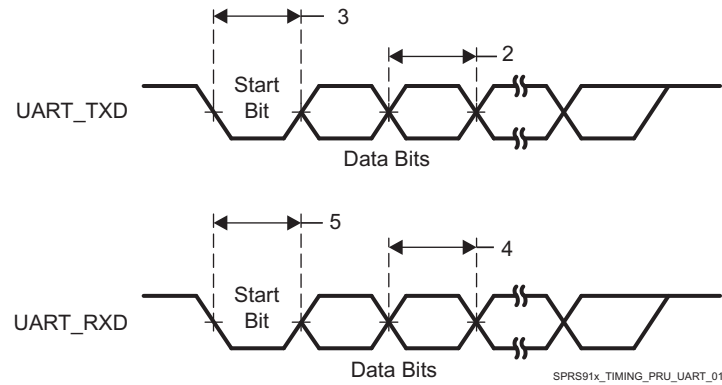
图 7-108. PRU-ICSS UART Timing
