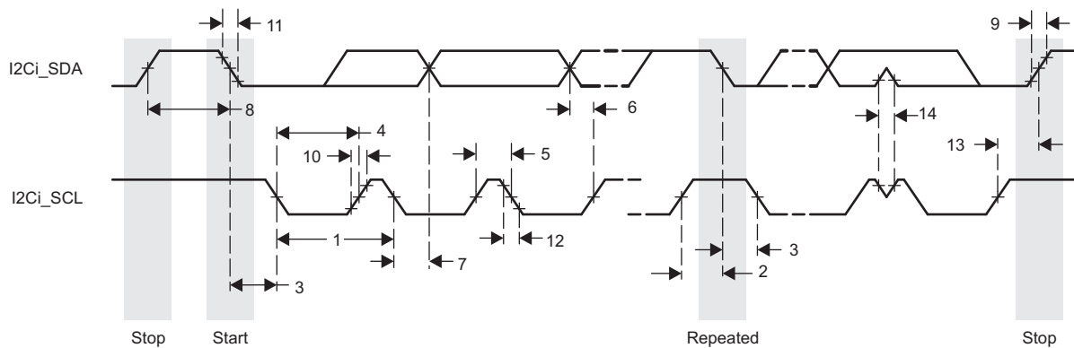
图 7-23. I2C Receive Timing
