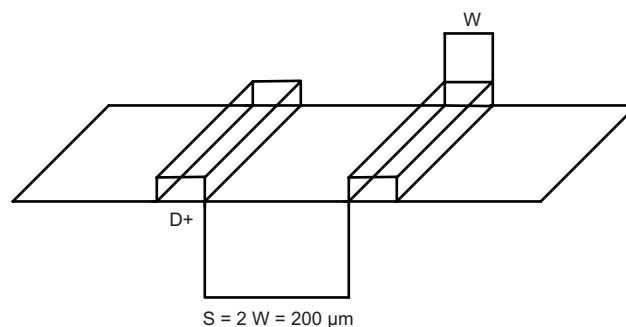
图 8-29. Ground Guard Illustration
