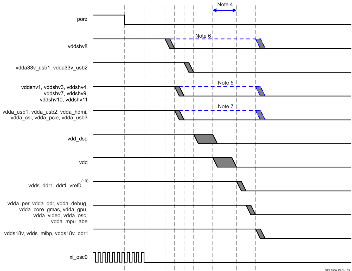
Figure 5-6. Power-Down Sequencing (8)(9)
