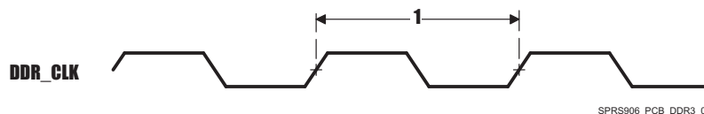
图 7-1. DDR3 Memory Controller Clock Timing
