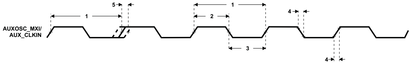
Figure 7-13. AUX_MXI/AUX_CLKIN Timing
