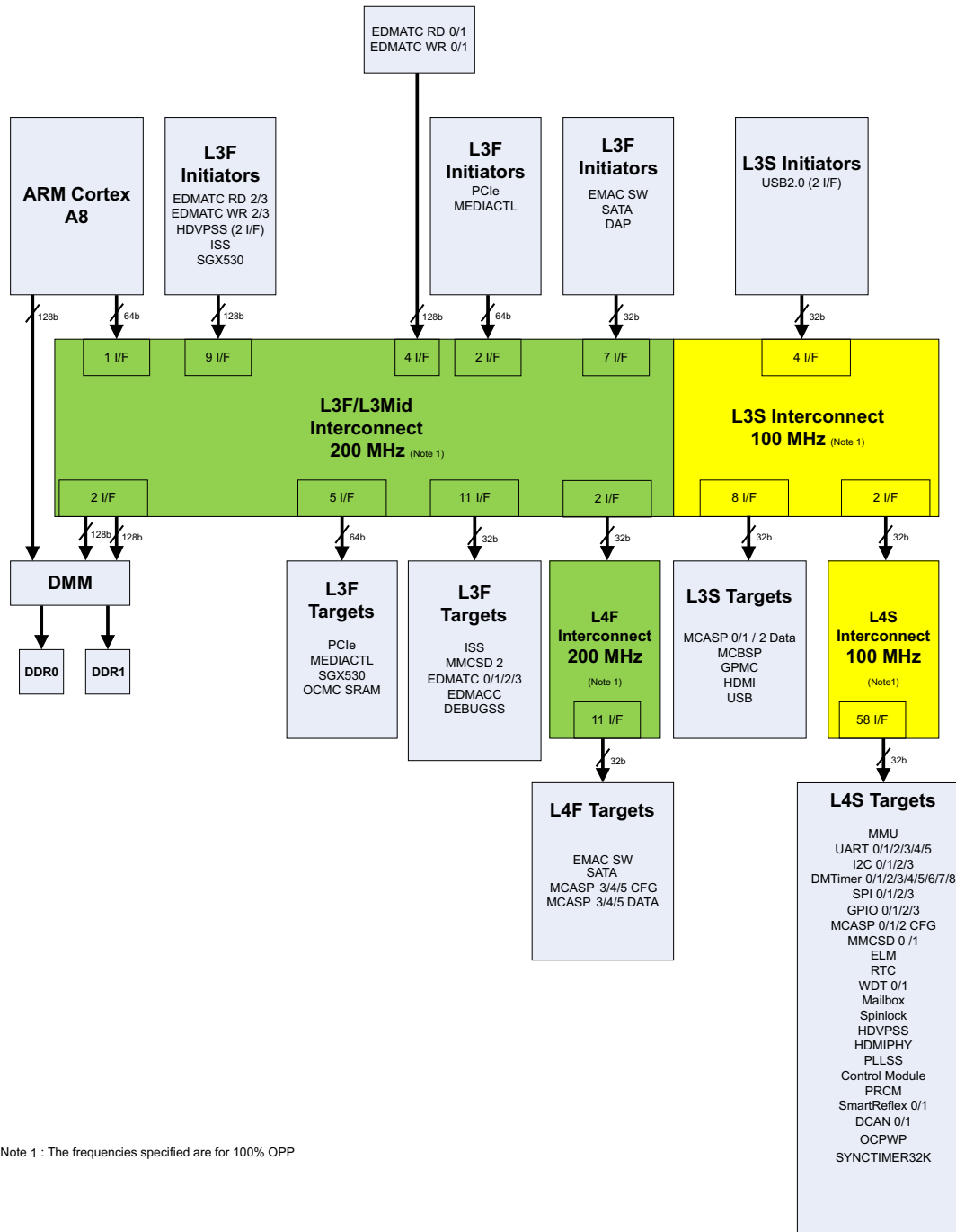
Figure 5-1. System Interconnect
