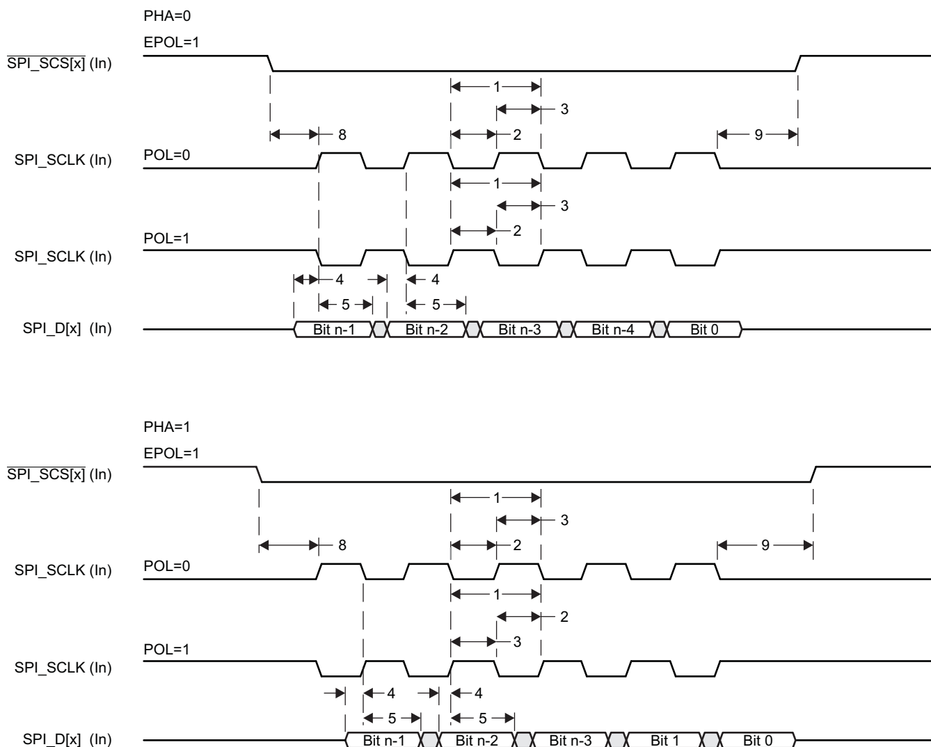
Figure 8-93. SPI Slave Mode Receive Timing
