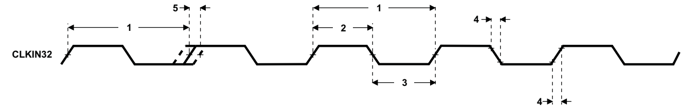
Figure 7-14. CLKIN32 Timing
