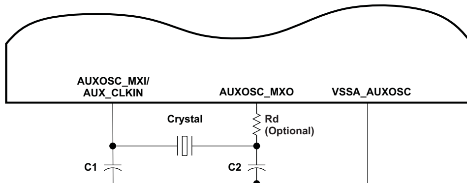
Figure 7-8. Auxiliary Oscillator
