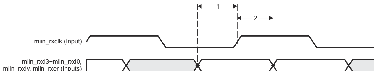
图 6-17. GMAC Receive Interface Timing MII operation
