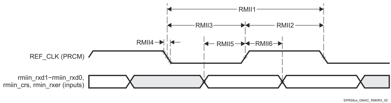
图 6-14. GMAC Receive Interface Timing RMIIn operation
