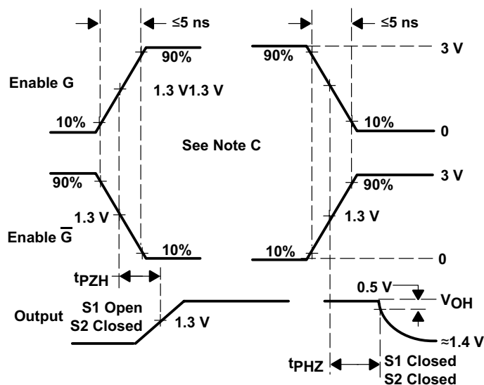
图 7-3. Voltage Waveforms For t_{PZH} , t_{PZH}
