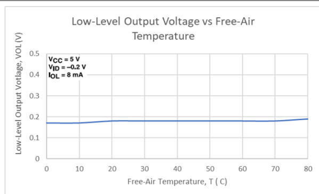
图 6-3. Low-Level Output Voltage vs Free-Air Temperature
