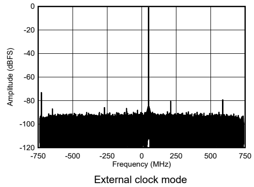
图 4-441. RX Single Tone Output FFT at 8.11GHz, -1dBFS
