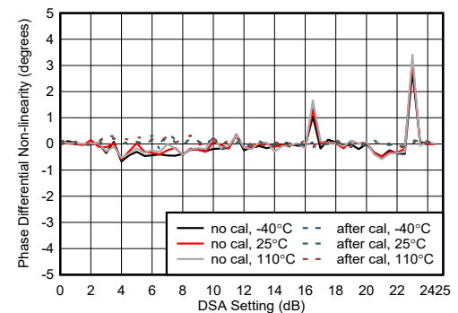
图 4-427. RX Phase Differential Nonlinearity at 8.11GHz
