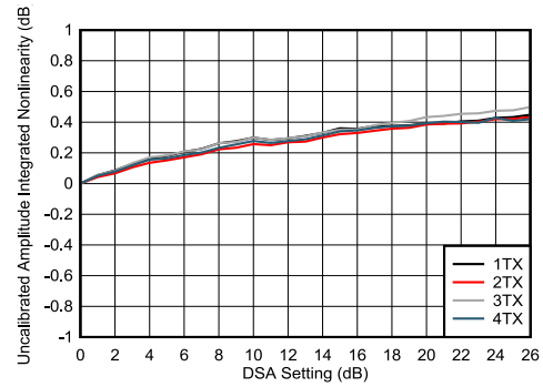
图 4-240. TX DSA Uncalibrated Amplitude Integrated Nonlinearity
