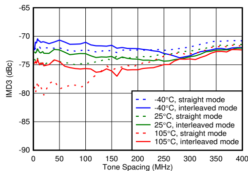
图 4-99. TX IMD3 vs Tone Spacing and Temperature at 2.6GHz
