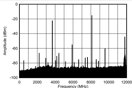
图 4-205. TX Single Tone Output Spectrum at 8.1GHz
