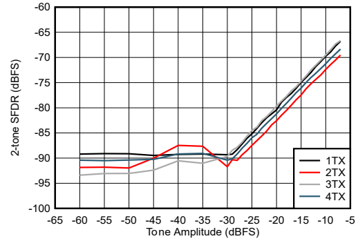
图 4-221. TX 2-Tone SFDR vs Digital Amplitude at 8.1GHz
