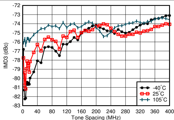
图 4-27. TX IMD3 vs Tone Spacing and Temperature at 0.85GHz
