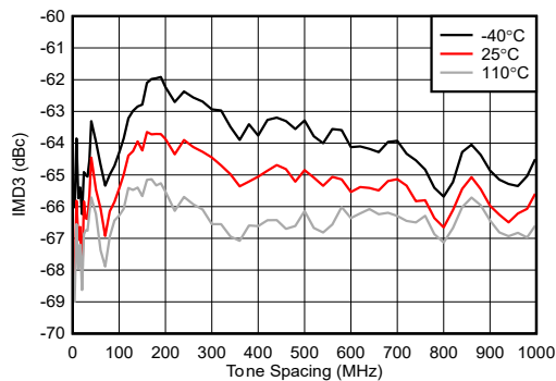
图 4-259. TX IMD3 vs Tone Spacing at 9.61GHz
