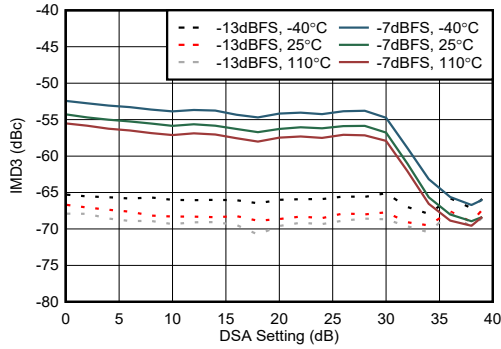
图 4-220. TX IMD3 vs DSA Setting at 8.1GHz
