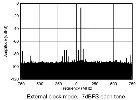
图 4-445. RX Dual Tone Output FFT at 8.11GHz
