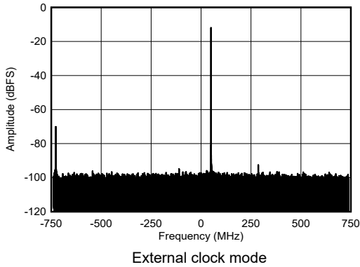
图 4-442. RX Single Tone Output FFT at 8.11GHz, -12dBFS
