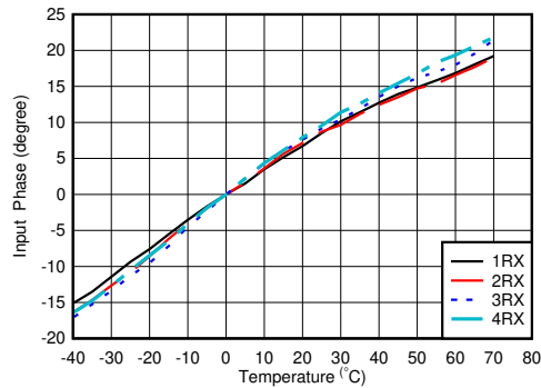
图 4-318. RX Input Phase vs Temperature and DSA at f_{\text{IN}} = 1.75\text{GHz}
