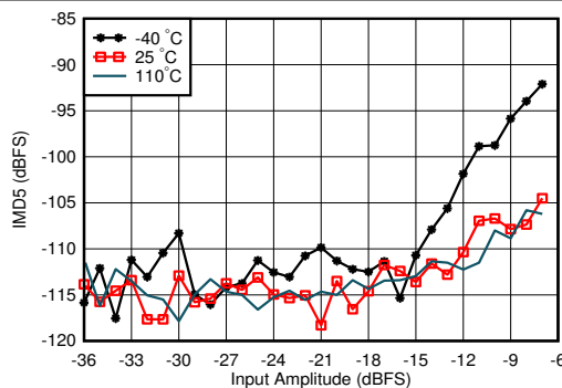
图 4-304. RX IMD5 vs Input Level and Temperature at 0.8GHz
