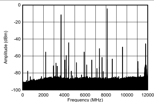
图 4-203. TX Single Tone Output Spectrum at 8.1GHz
