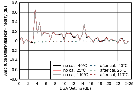
图 4-425. RX Amplitude Differential Nonlinearity at 8.11GHz
