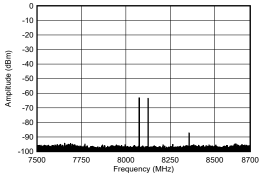
图 4-214. TX Dual Tone Output Spectrum at 8.11GHz
