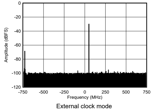
图 4-443. RX Single Tone Output FFT at 8.11GHz, -30 dBFS
