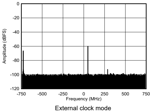
图 4-444. RX Single Tone Output FFT at 8.11GHz, -60 dBFS
