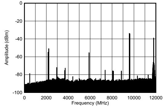
图 4-276. TX 2-Tone Spectrum at 9.61GHz and -30dBFS Each (wideband)
