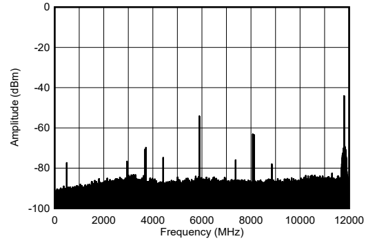
图 4-215. TX Dual Tone Output Spectrum at 8.11GHz
