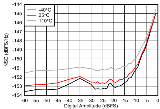
图 4-261. TX NSD vs Digital Amplitude at 9.61GHz
