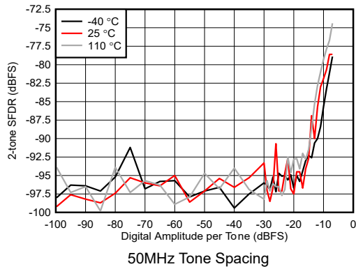
图 4-440. RX 2-tone SFDR vs Digital Amplitude at 8.11GHz
