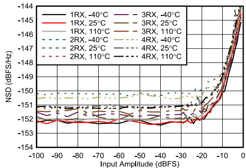
图 4-432. RX NSD vs Digital Amplitude at 8.1GHz
