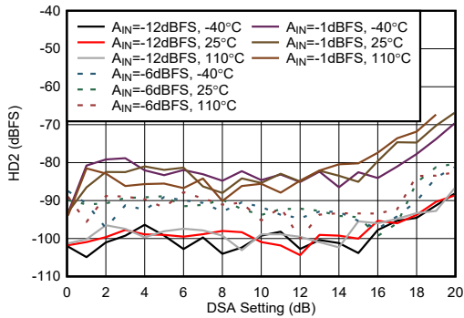
图 4-463. RX HD2 vs DSA Setting at 9.6GHz
