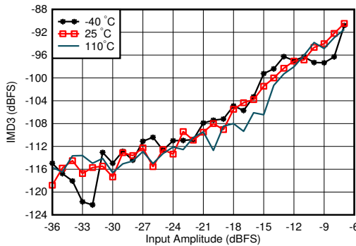
图 4-332. RX IMD3 vs Input Level and Temperature at 1.75GHz
