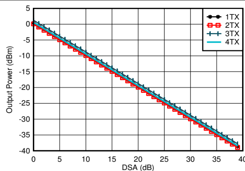
图 4-119. TX Output Power vs DSA Setting at 3.5GHz
