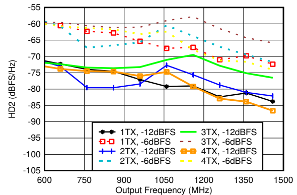
Matching at 0.8GHz, f_{DAC} = 8847.36\text{GSPS} , straight mode
