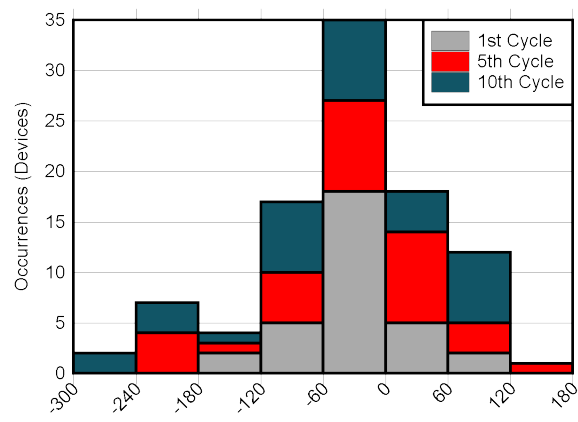
– 40°C to +85°C cycles, 60 minutes per cycle
