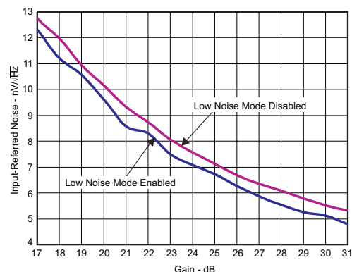
Figure 8. Input-Referred Noise for High Gains
