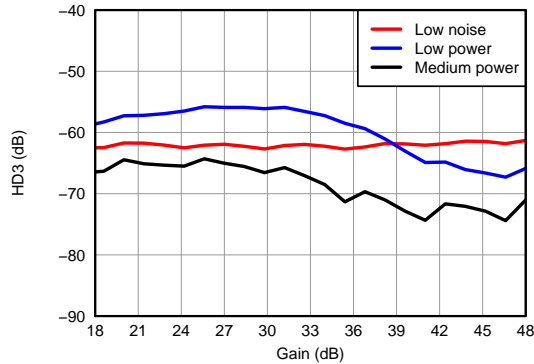
Figure 44. HD3 vs Gain
