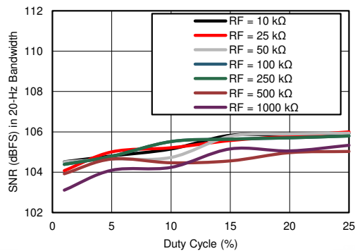
图 7-15. Receiver SNR in 20-Hz BW vs Duty Cycle (Different Gain Settings)
