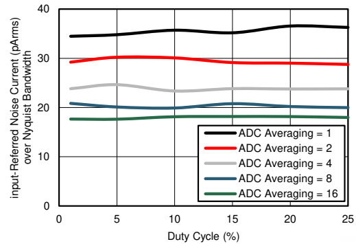
图 7-18. Receiver Input-Referred Noise Current over Nyquist Bandwidth vs Duty Cycle (Different ADC Averaging)
