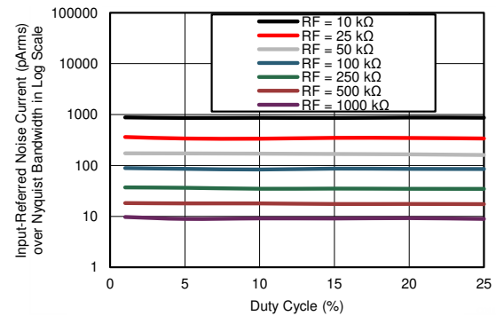
图 7-14. Receiver Input-Referred Noise Current over Nyquist Bandwidth vs Duty Cycle (Different Gain Settings)
