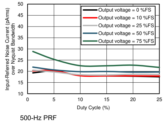
图 7-12. Input-Referred Noise Current over Nyquist Bandwidth vs Duty Cycle (Input Current with Tx-Rx Loopback)
