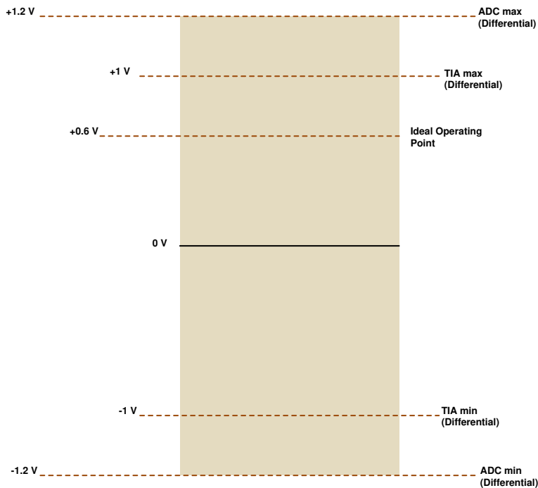
图 8-3. Signal Levels in TIA and ADC
