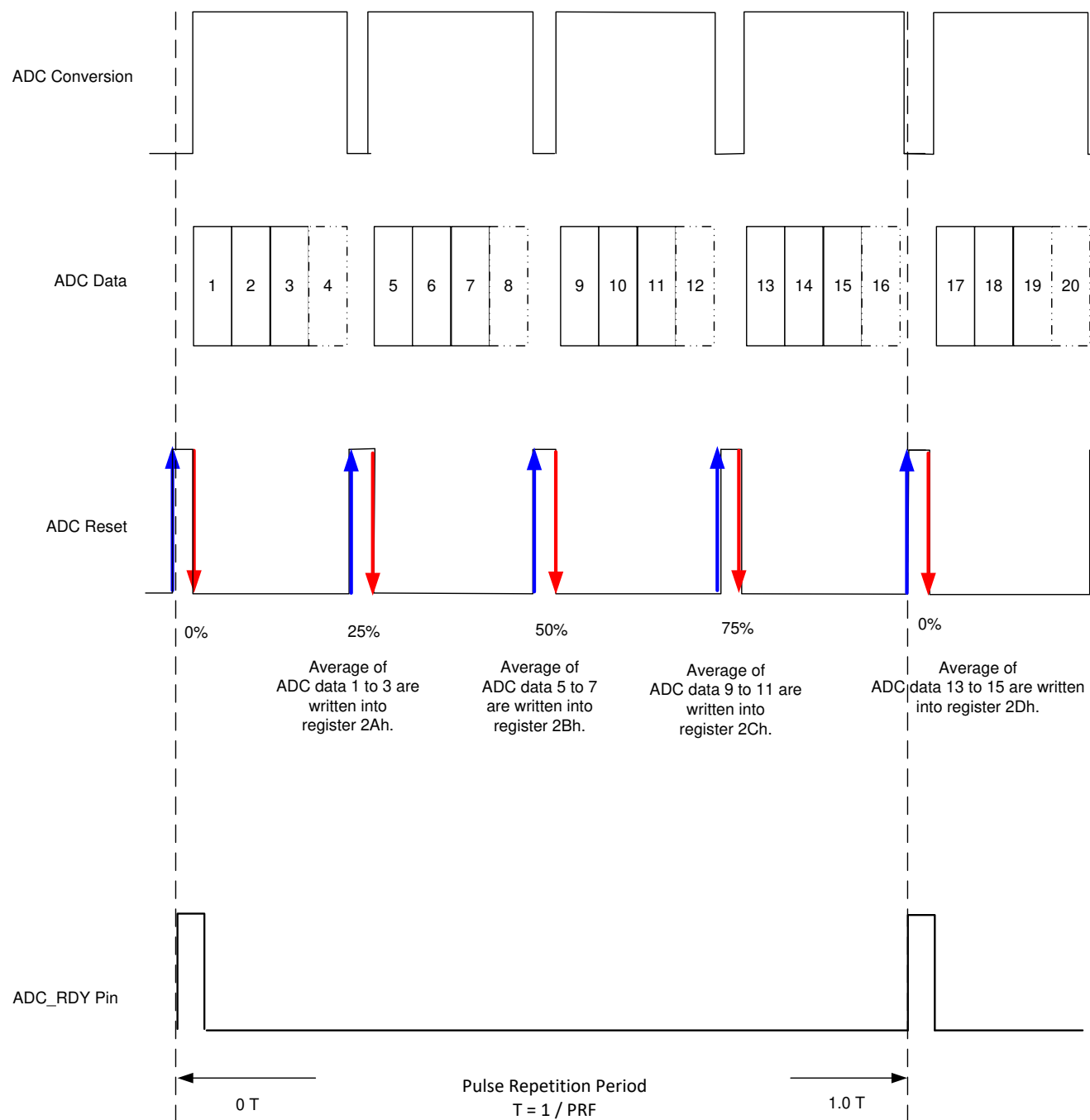
图 8-29. ADC Data with Averaging Enabled
