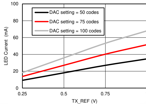
图 7-35. Transmitter Current vs TX_REF Voltage (Multiple DAC Settings)
