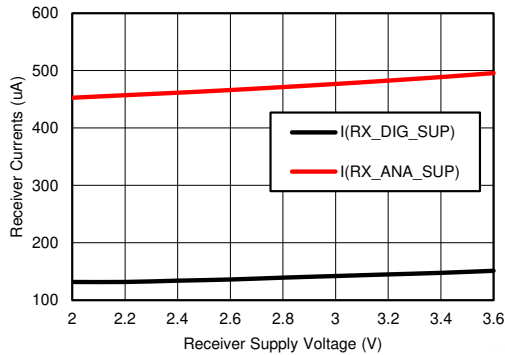
图 7-5. Receiver Currents vs Receiver Supply Voltage
