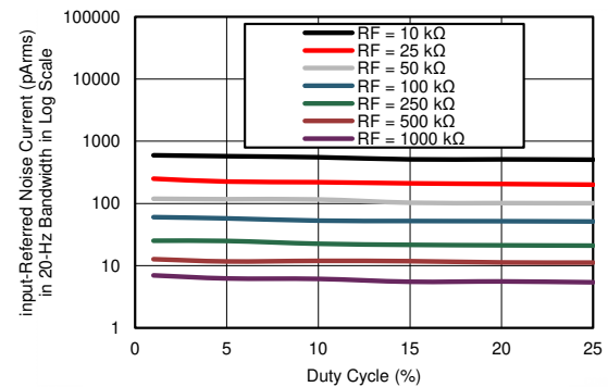
图 7-16. Receiver Input-Referred Noise Current in 20-Hz BW vs Duty Cycle (Different Gain Settings)
