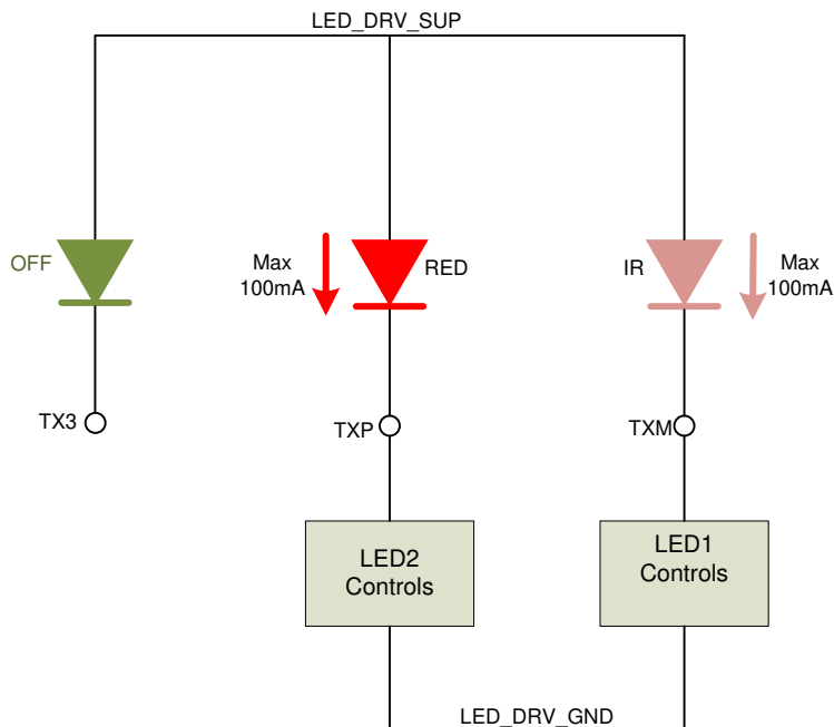
图 8-21. SPO2 Application, Common Anode Configuration
