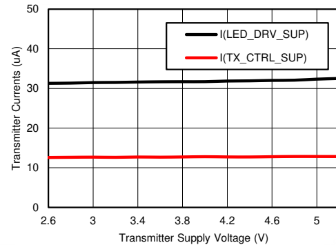
图 7-6. Transmitter Currents vs Transmitter Supply Voltage
