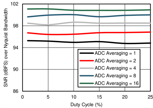
图 7-17. Receiver SNR over Nyquist Bandwidth vs Duty Cycle (Different ADC Averaging)
