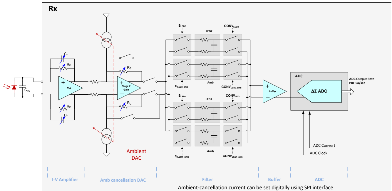
图 8-1. Receiver Front-End
