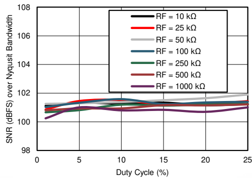
图 7-13. Receiver SNR over Nyquist Bandwidth vs Duty Cycle (Different Gain Settings)
