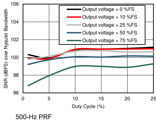
图 7-11. SNR over Nyquist Bandwidth vs Duty Cycle (Input Current with Tx-Rx Loopback)
