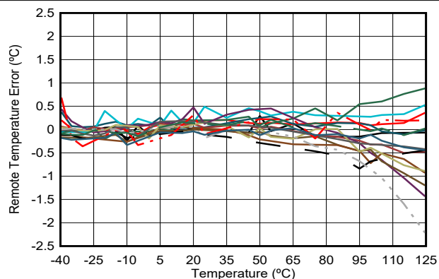
图 6-49. Remote Temperature Error vs Temperature
