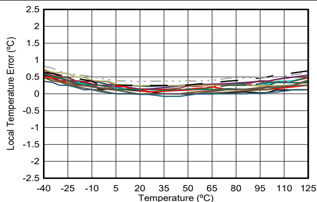
图 6-48. Local Temperature Error vs Temperature
