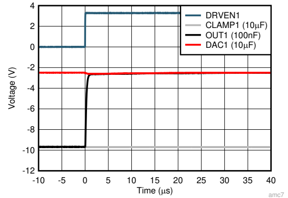
DAC 输出: -2.5V C_L = 100\text{nF} CLAMP 输出: -9.6875V
