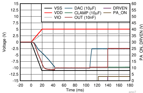
DAC 输出: -2.5V CLAMP 输出: -9.6875V
