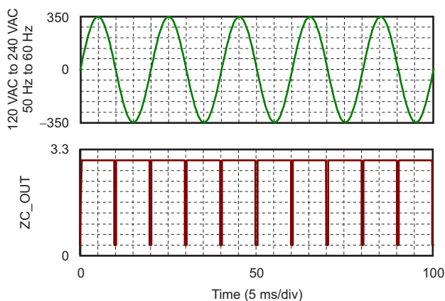
Figure 21. Isolated Zero-Crossing Waveforms
