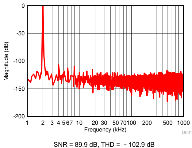
图 8-3. Typical FFT With a 2-kHz Signal
