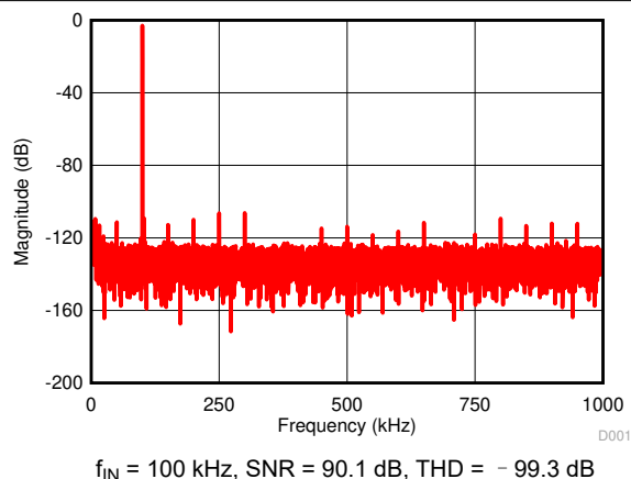
图 6-4. Typical FFT at f_{\text{IN}} = 100\text{ kHz}
