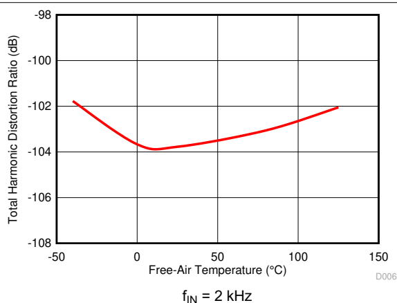
图 6-8. THD vs Free-Air Temperature
