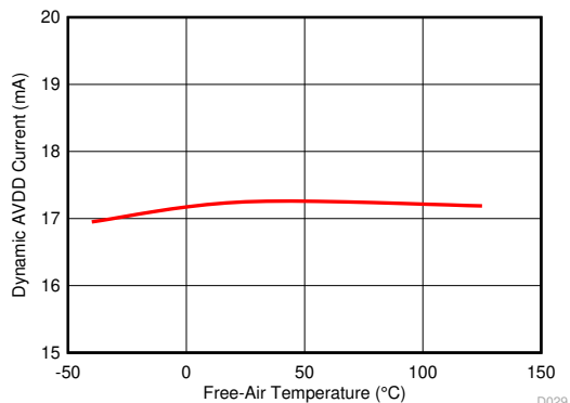
图 6-22. Dynamic AVDD Current vs Free-Air Temperature
