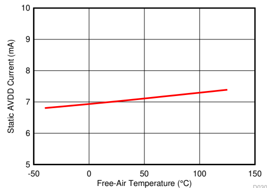
图 6-23. Static AVDD Current vs Free-Air Temperature
