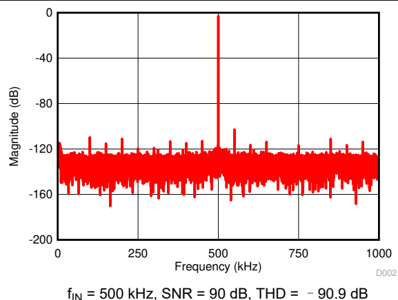
图 6-5. Typical FFT at f_{\text{IN}} = 500\text{ kHz}
