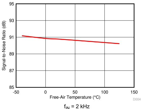
图 6-6. SNR vs Free-Air Temperature
