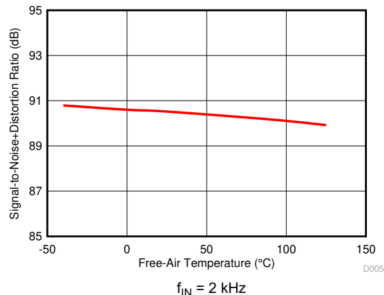
图 6-7. SINAD vs Free-Air Temperature
