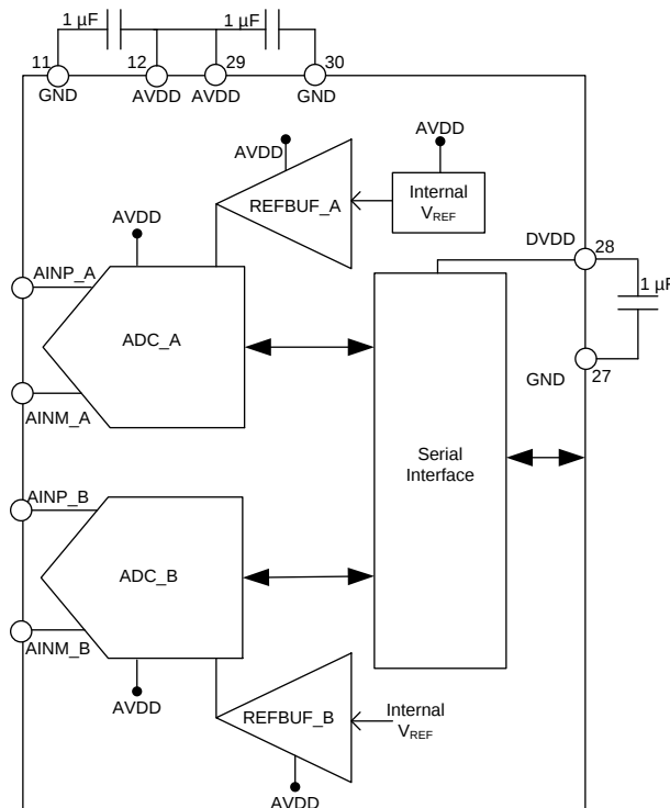
图 83. Power-Supply Decoupling
