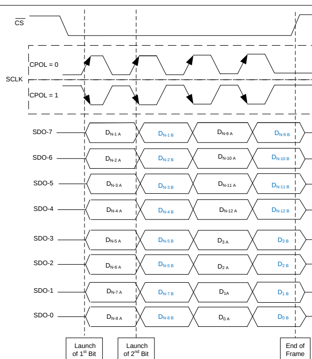
图 63. PB-01-AB-SDR and PB-11-AB-SDR Protocols
