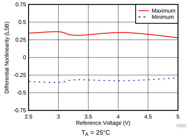
Figure 14. DNL vs Reference Voltage
