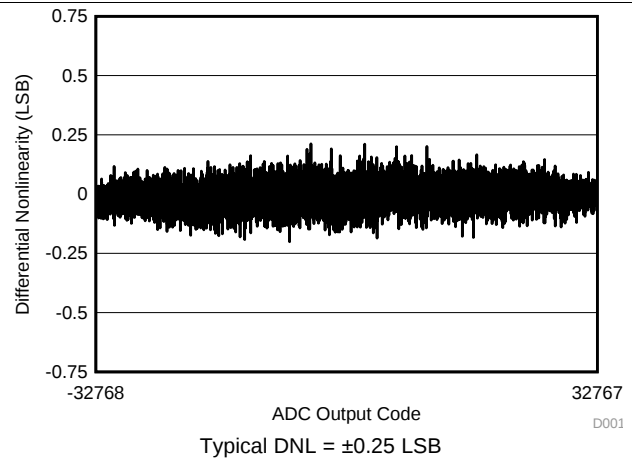
Figure 8. Typical DNL
