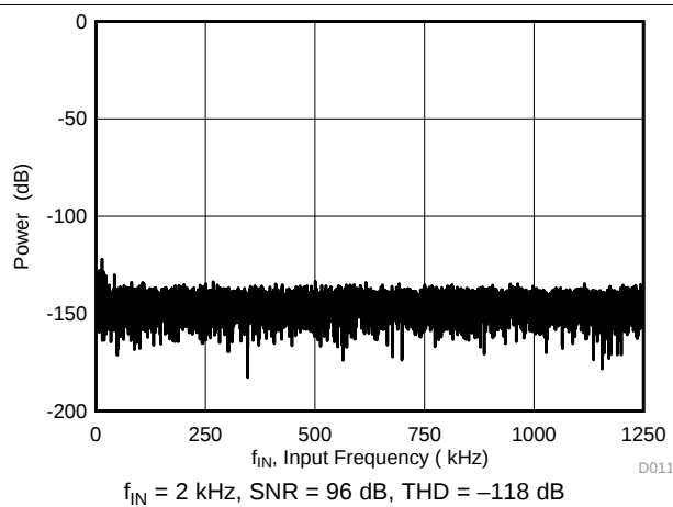
Figure 17. Typical FFT
