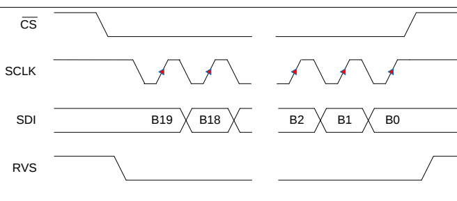
Figure 55. SPI-11-S Protocol, Optimal Command Frame
