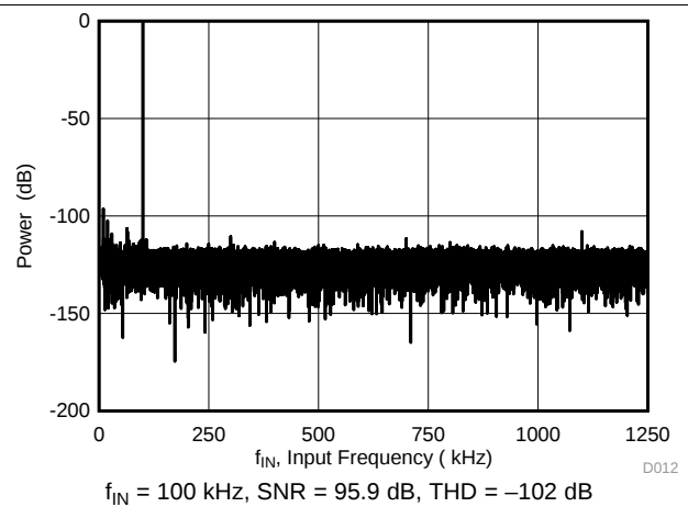
Figure 18. Typical FFT
