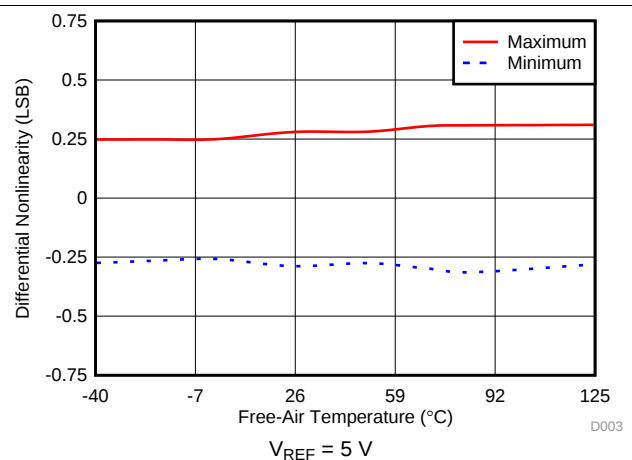
Figure 12. DNL vs Temperature
